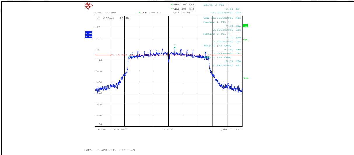
11G_ANT2_2437_6dB Bandwidth
