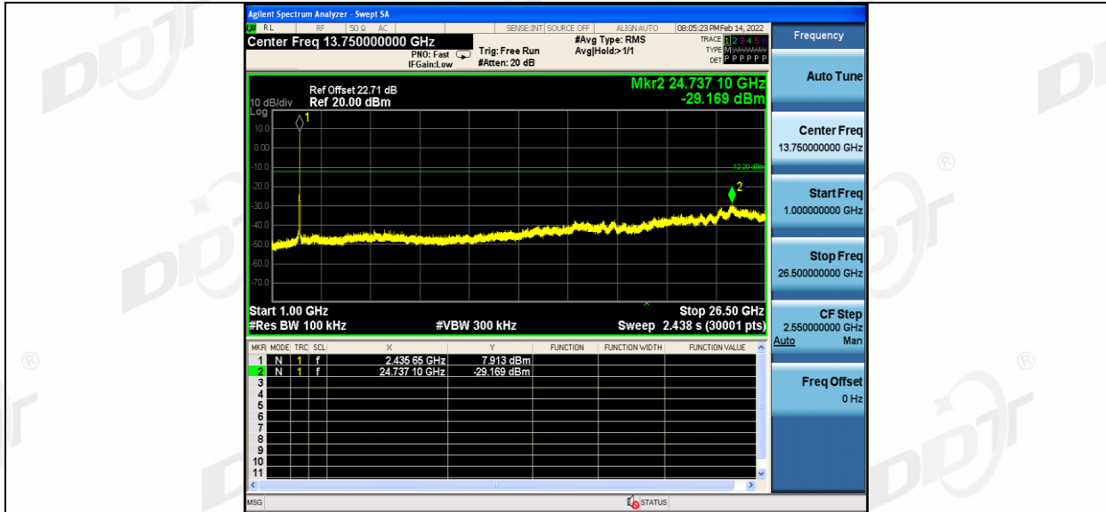
11AX20SU_Ant2_2437_0-Reference
