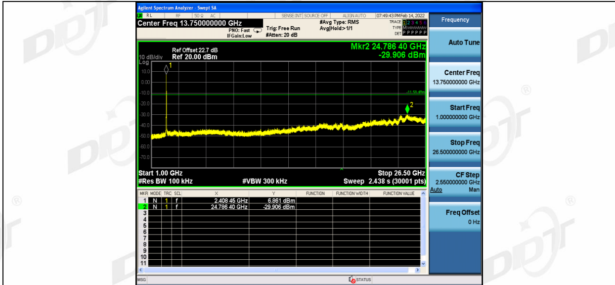
11AX20SU_Ant2_2412_0-Reference
