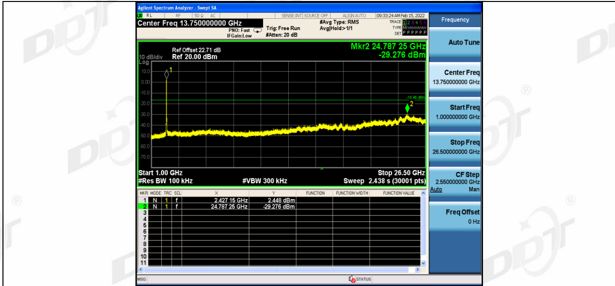
11AX40SU_Ant2_2422_0-Reference
