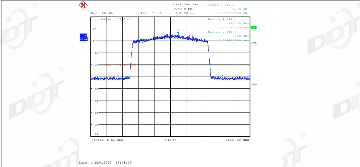
11AX40SU_Ant2_5510
