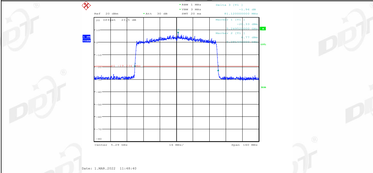
11AX80SU_Ant2_5290
