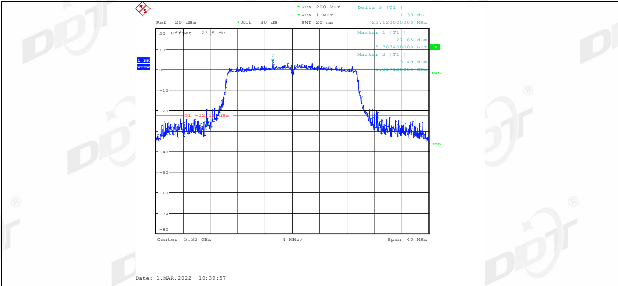
11AX20SU_Ant2_5320
