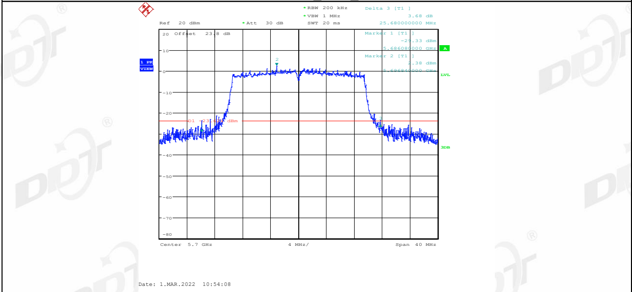
11AX20SU_Ant1_5745
