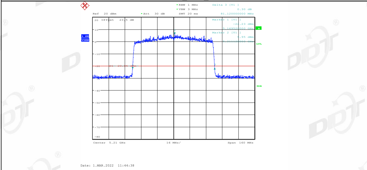
11AX80SU_Ant2_5210
