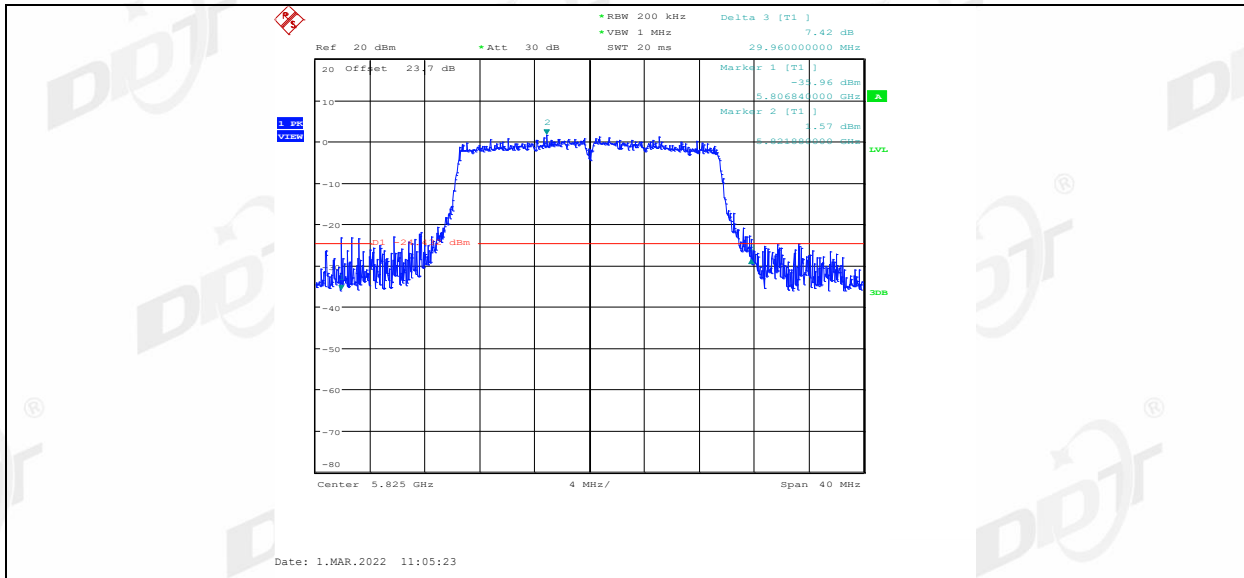
11AX20SU_Ant2_5825
