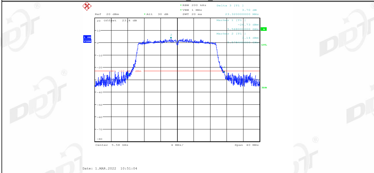
11AX20SU_Ant2_5580
