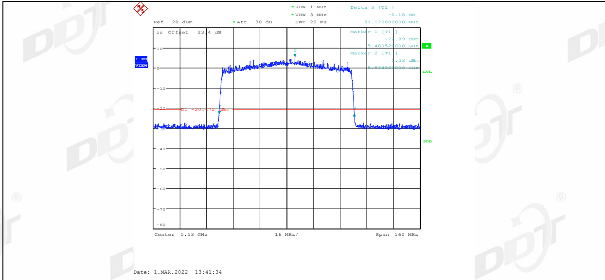
11AX80SU_Ant2_5530
