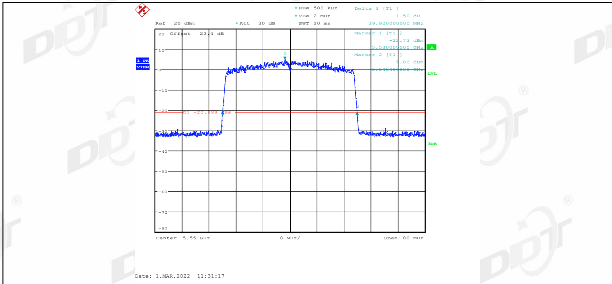
11AX40SU_Ant2_5550
