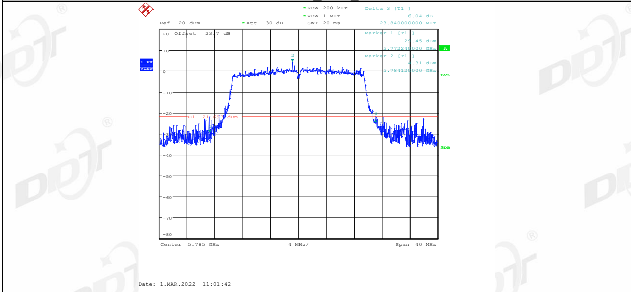
11AX20SU_Ant2_5785
