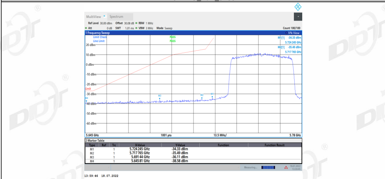
11AX40MIMO_High_5795
