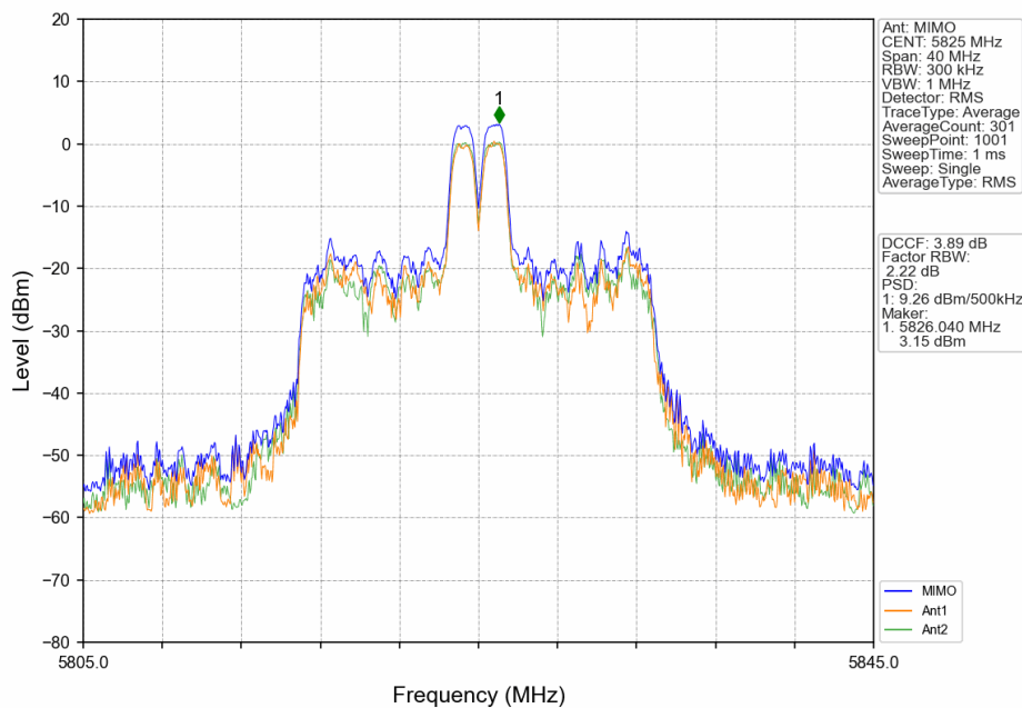
802.11ax(HEW20)_HCH_5825MHz_RU26_Mid_MIMO_NTNV
