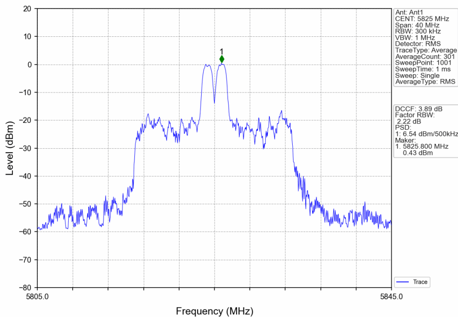
802.11ax(HEW20)_HCH_5825MHz_RU26_Mid_Ant1_NTNV
