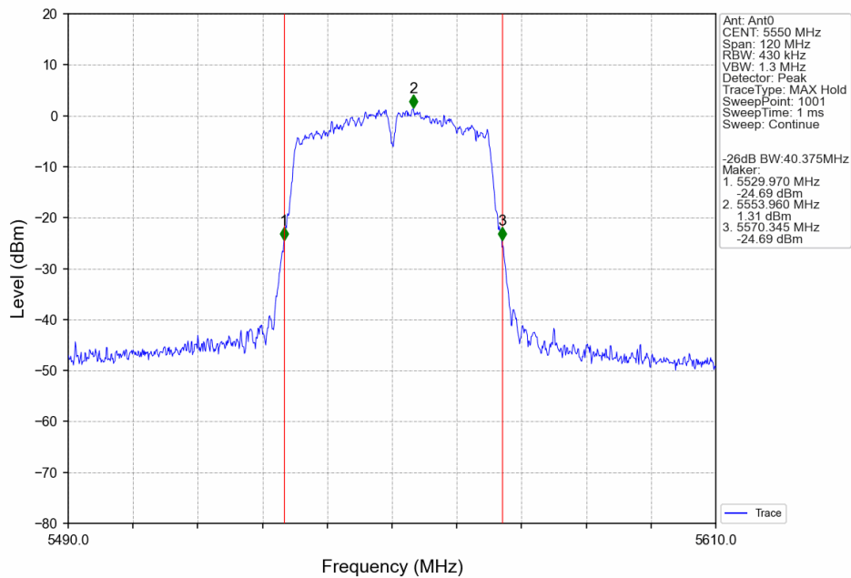
802.11ac(VHT40)_MCH_5550MHz_Ant0_NTNV
