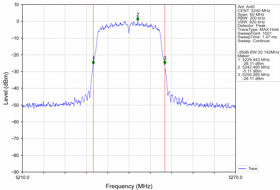
802.11ac(VHT20)_HCH_5240MHz_Ant0_NTNV
