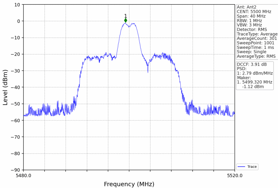
802.11ax(HEW20)_LCH_5500MHz_RU26_Mid_Ant2_NTNV
