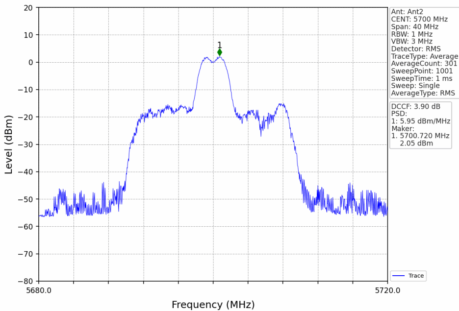
802.11ax(HEW20)_HCH_5700MHz_RU26_Mid_Ant2_NTNV
