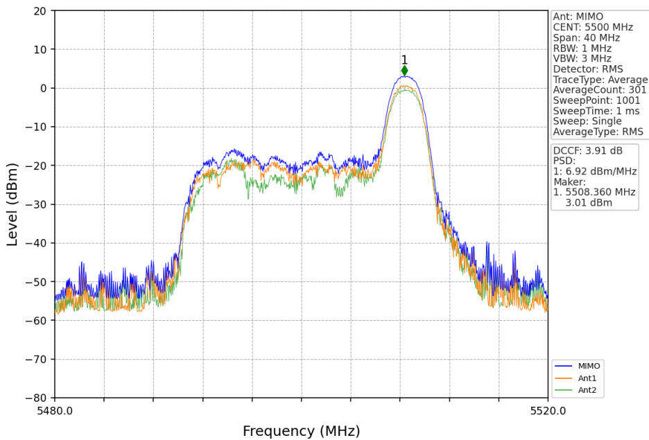
802.11ax(HEW20)_LCH_5500MHz_RU26_Right_MIMO_NTNV
