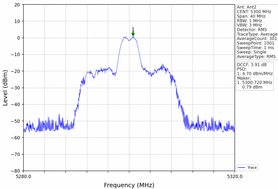
802.11ax(HEW20)_MCH_5300MHz_RU26_Mid_Ant2_NTNV
