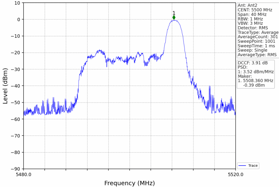
802.11ax(HEW20)_LCH_5500MHz_RU26_Right_MIMO_NTNV
