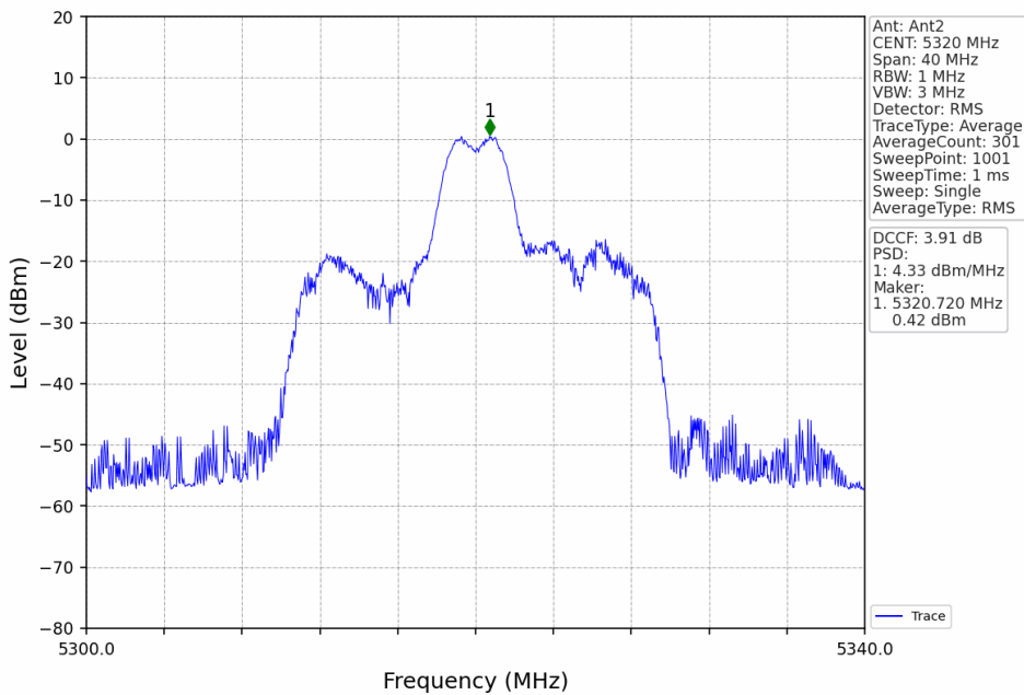
802.11ax(HEW20)_HCH_5320MHz_RU26_Mid_Ant2_NTNV
