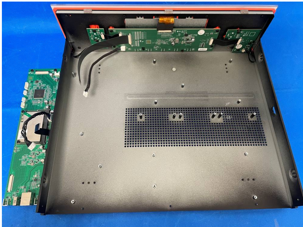
Figure 6. Internal view 5
