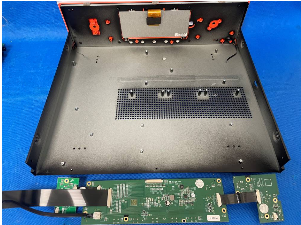
Figure 7. Internal view 6
