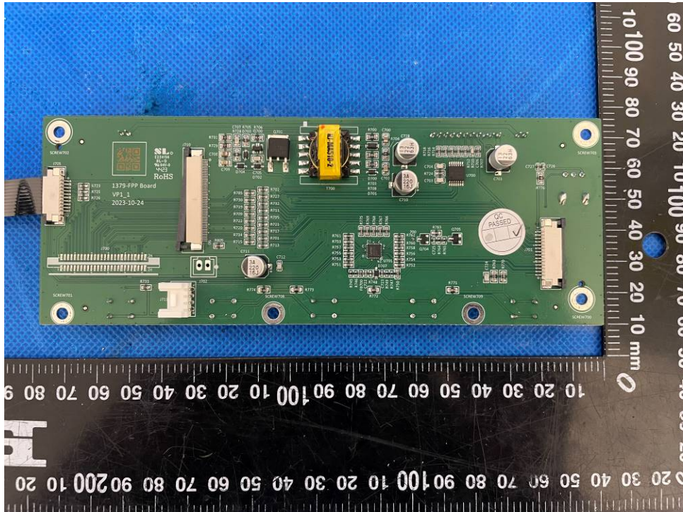
Figure 17. FFP board view 2
