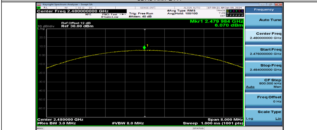
3DH5-Ant1-2480
