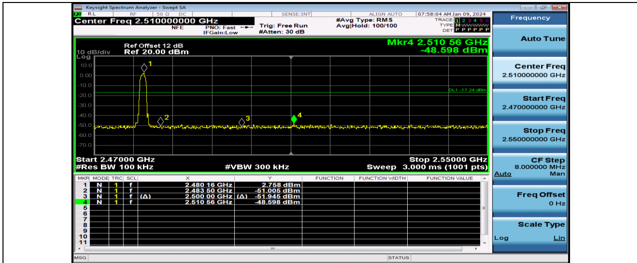
3DH5-Ant1-2480
