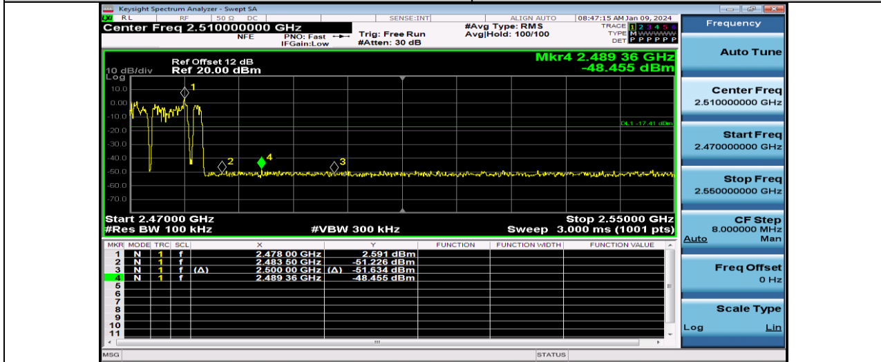
2DH5-Ant1-Hop_2480
