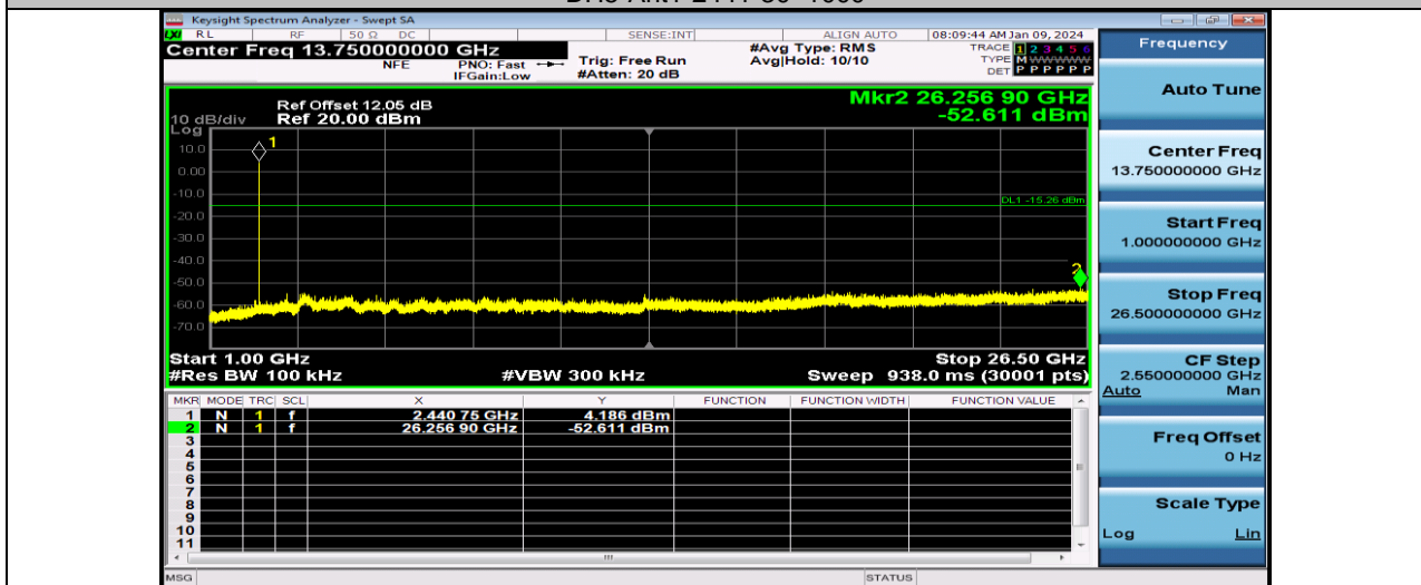
DH5-Ant1-2441-1000~26500
