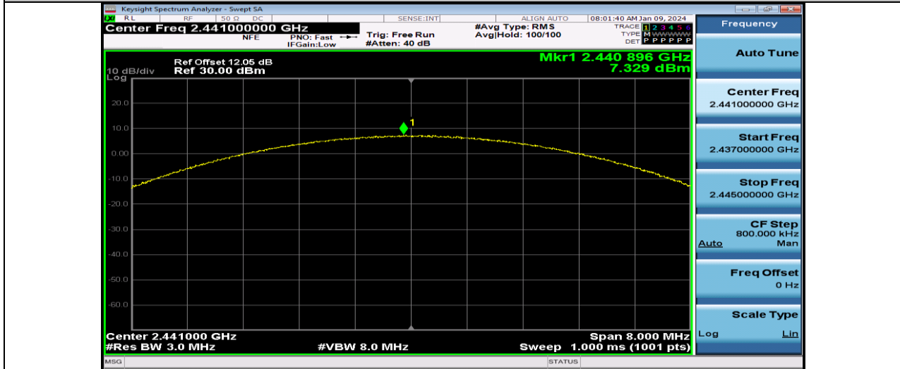
3DH5-Ant1-2441
