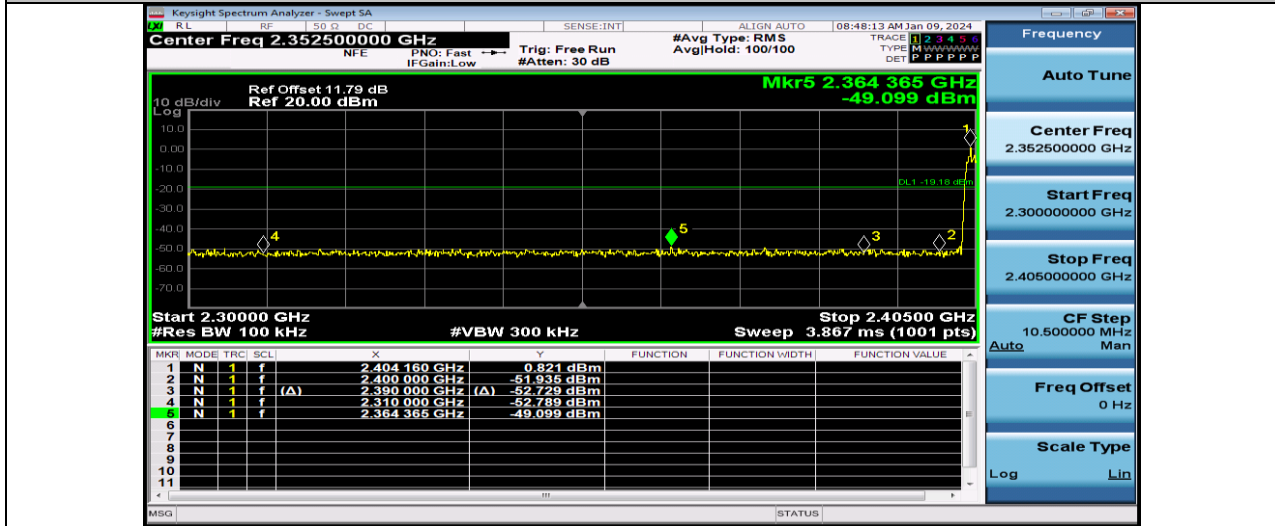
3DH5-Ant1-Hop_2402
