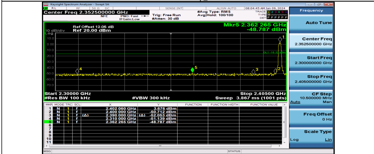
3DH5-Ant1-2402
