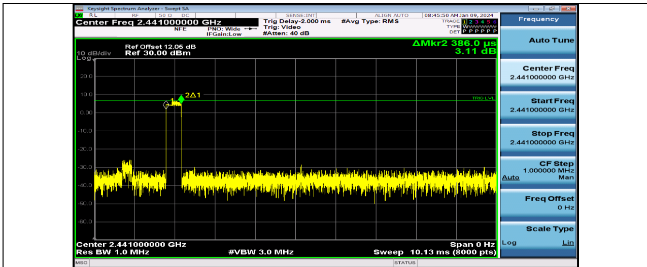
2DH1-Ant1-Hop
