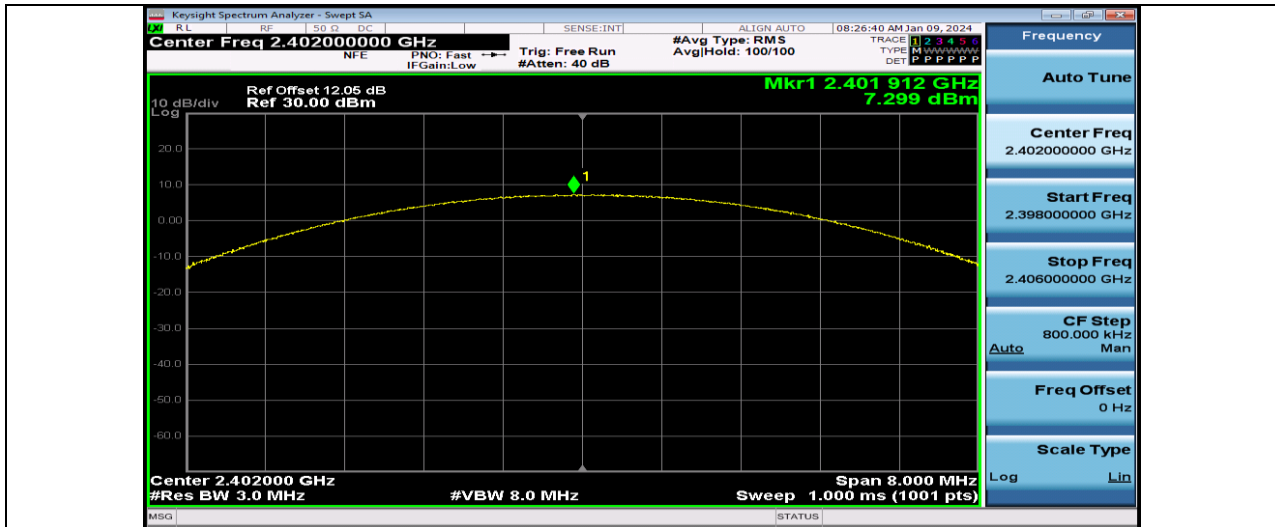
2DH5-Ant1-2402
