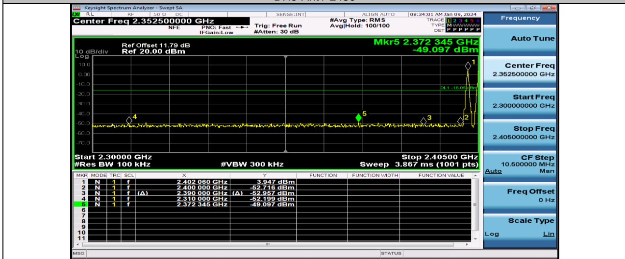
DH5-Ant1-Hop_2402
