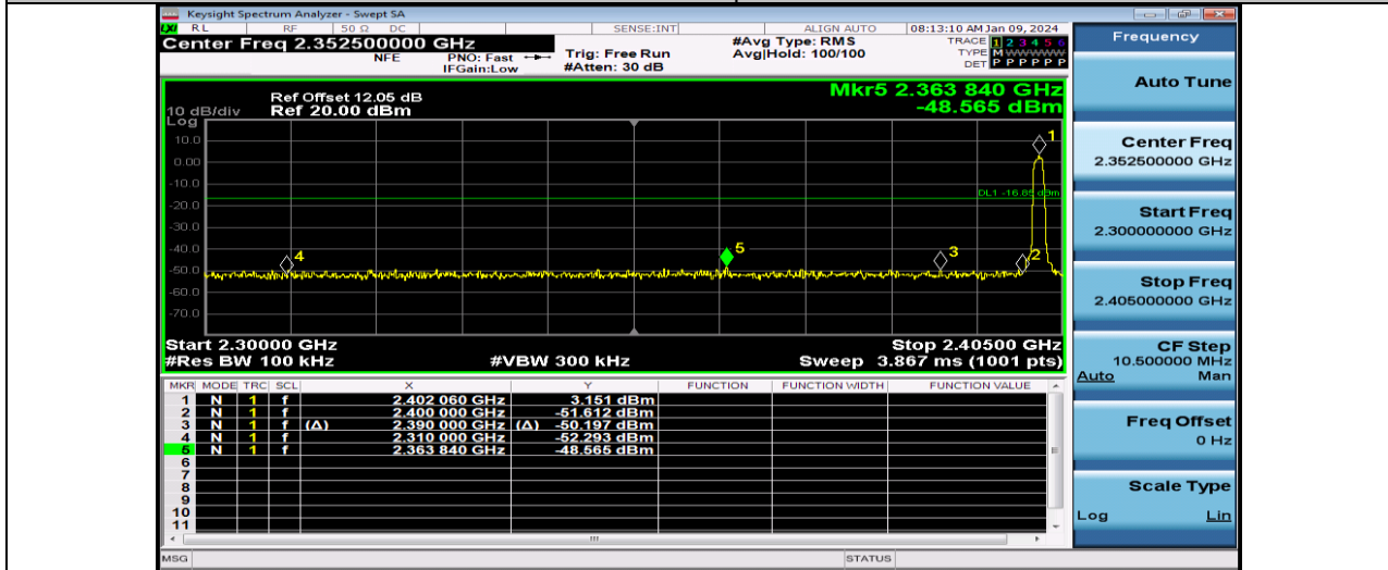
2DH5-Ant1-2402
