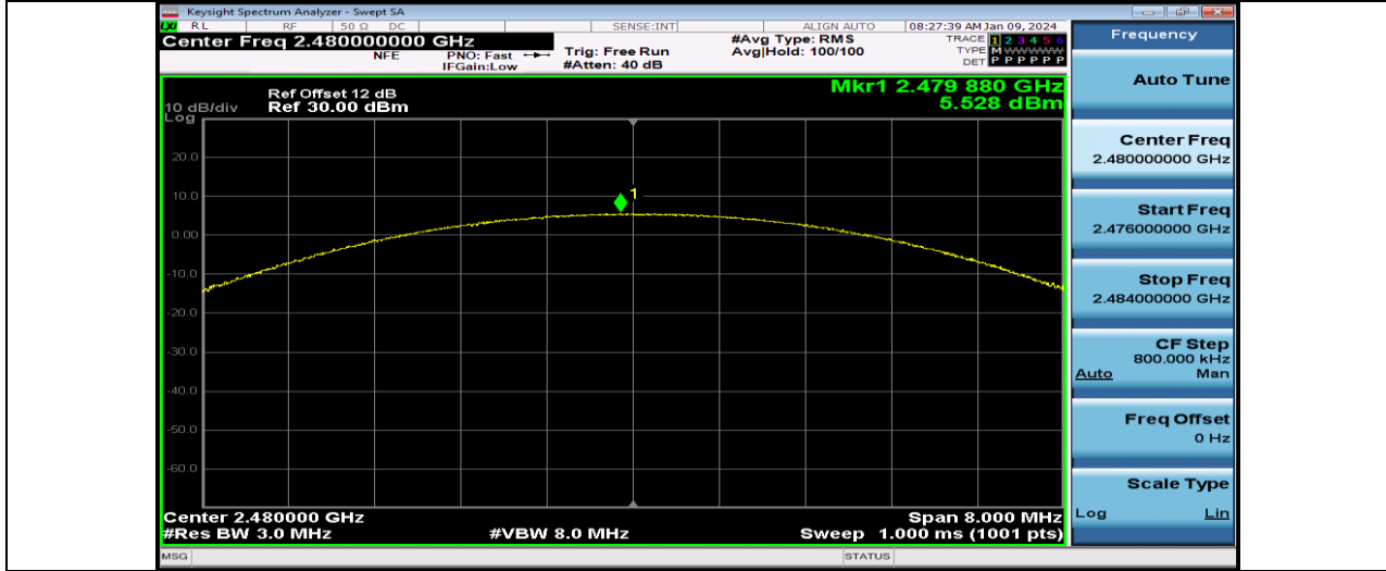
2DH5-Ant1-2480
