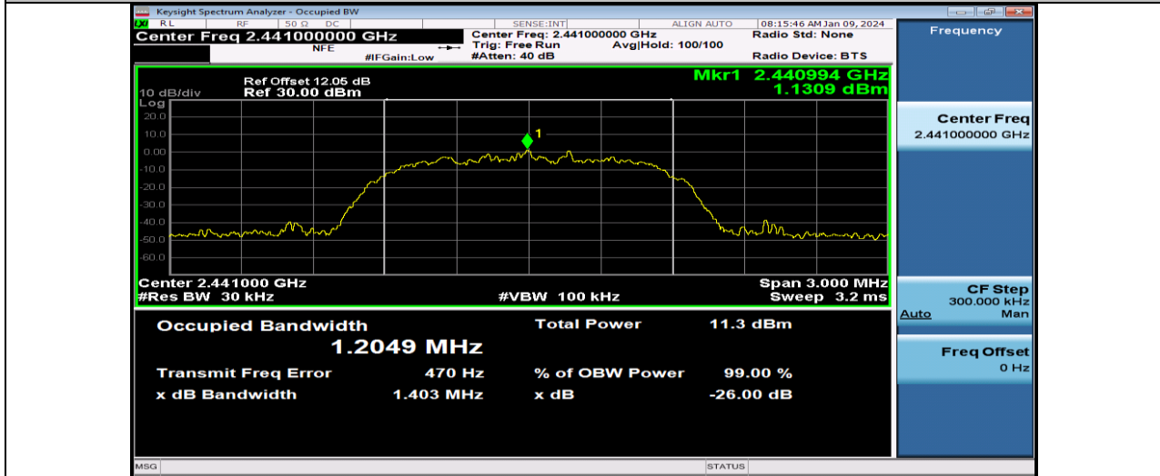
2DH5-Ant1-2441
