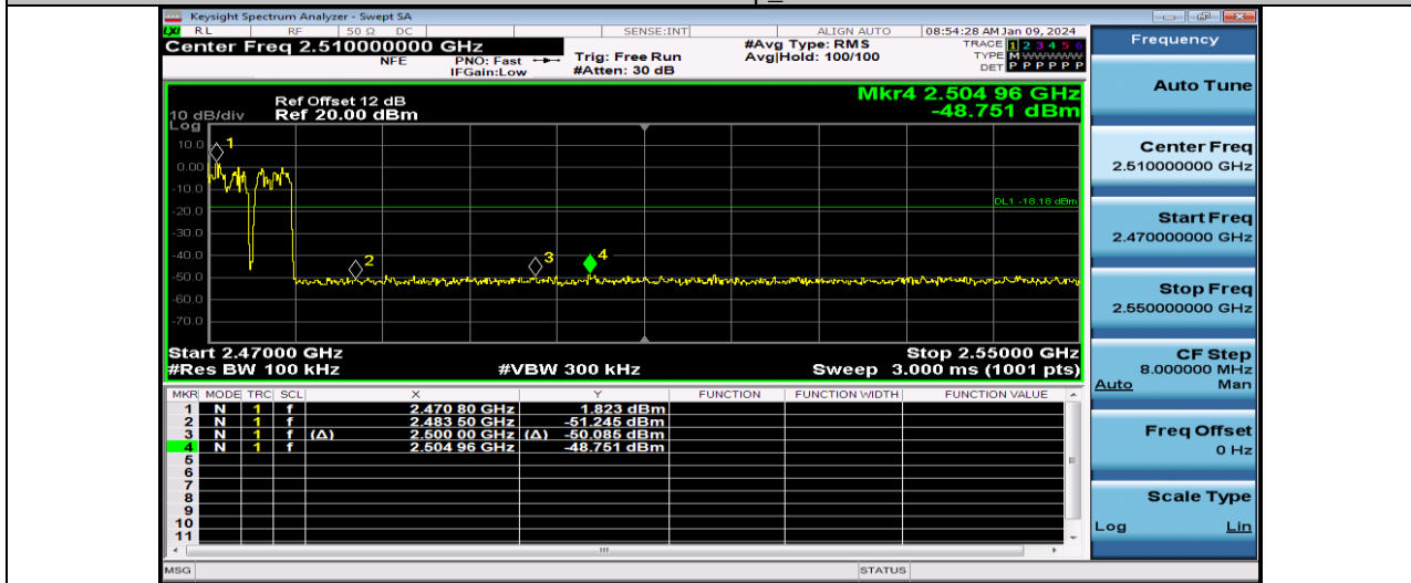
3DH5-Ant1-Hop_2480
