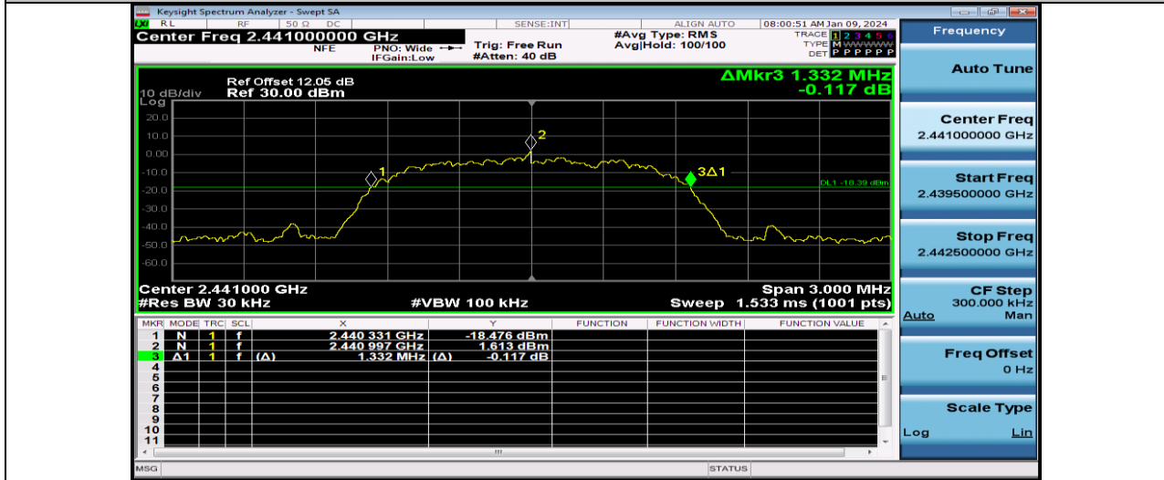
3DH5-Ant1-2441
