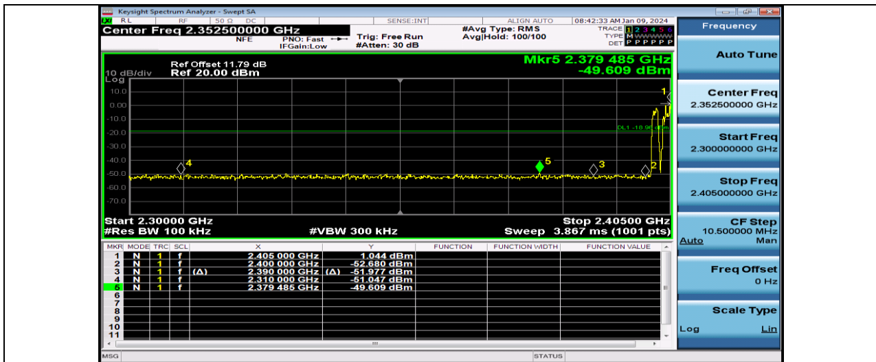
2DH5-Ant1-Hop_2402
