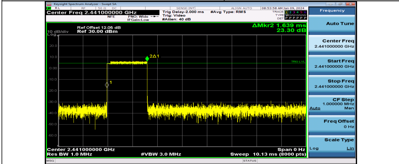
2DH3-Ant1-Hop
