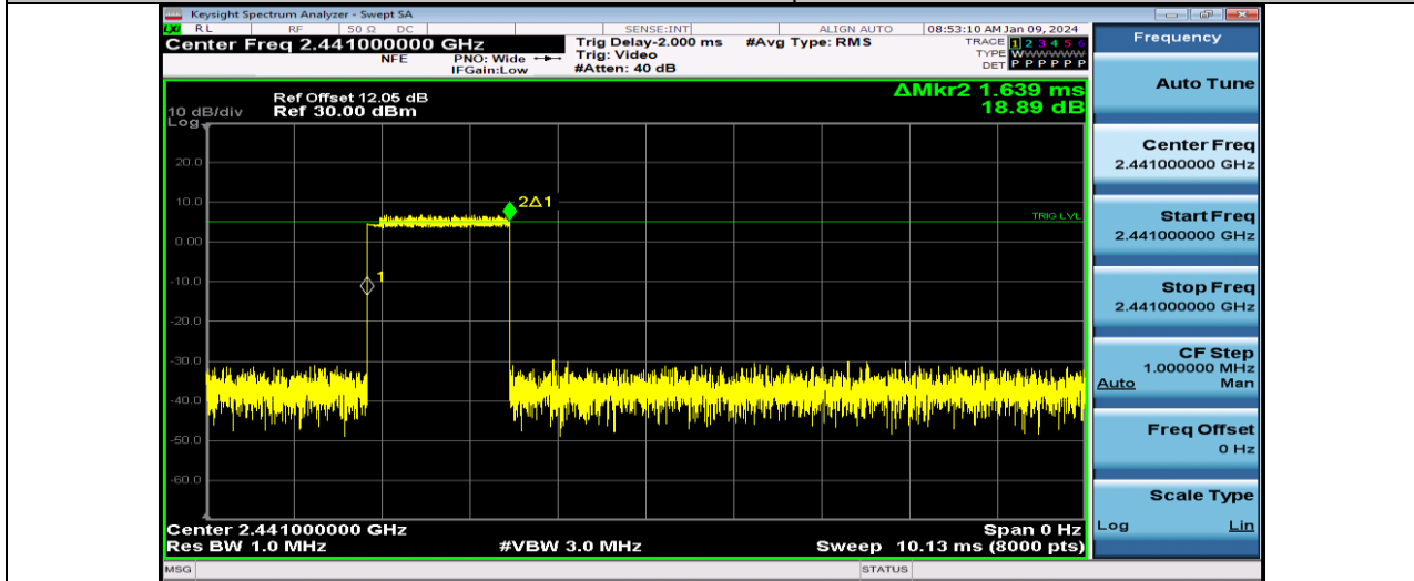
3DH3-Ant1-Hop
