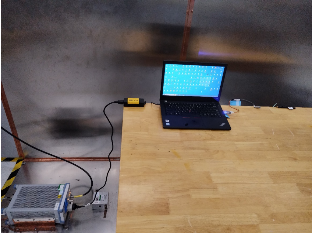
Photograph 3: Set-up for Conducted Emission
