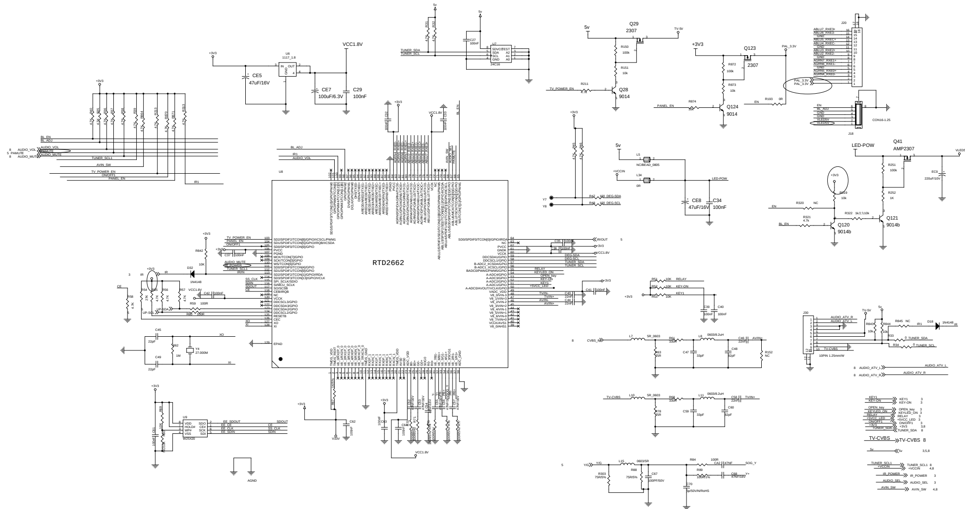
RTD2660 General GPIO List
