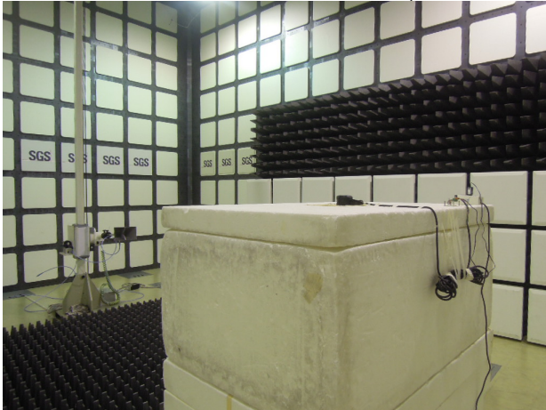
FCC_15_247_SRD_Radiated_Setup
