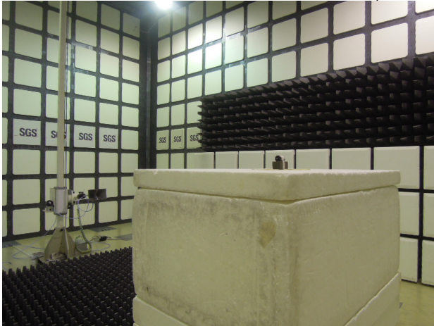
FCC 15 247 SRD Radiated_RC-K3X-001HJ_Setup
