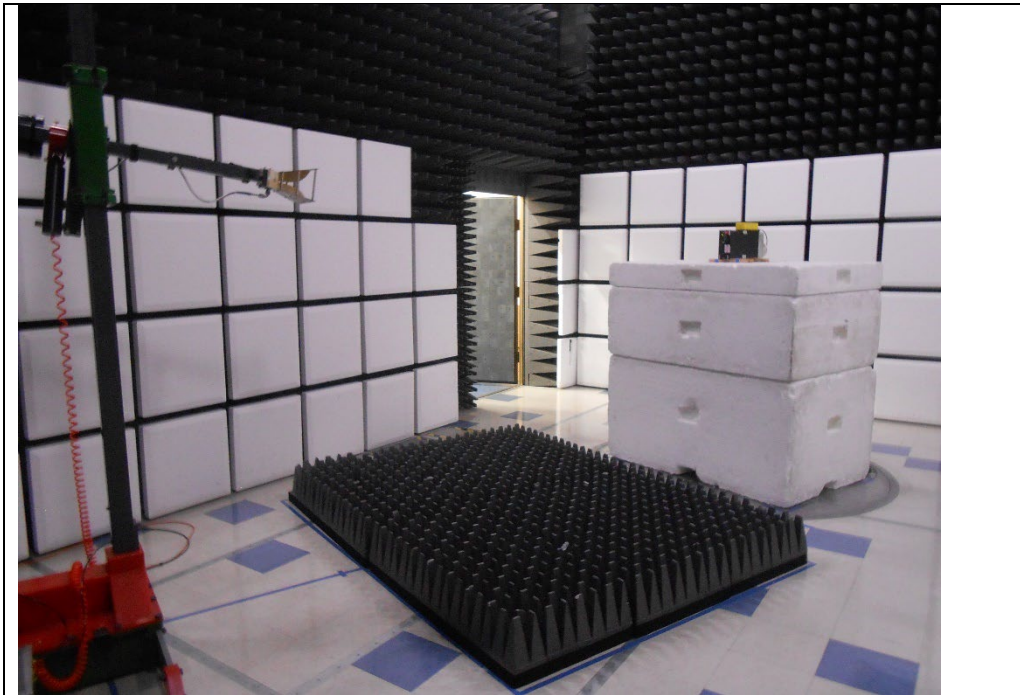
RF Radiated_ 1000 – 1500 MHz_#2
