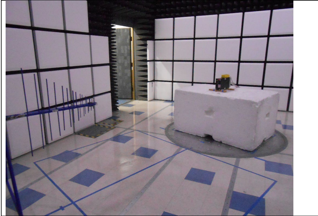
RF Radiated 30 – 1000 MHz #2
