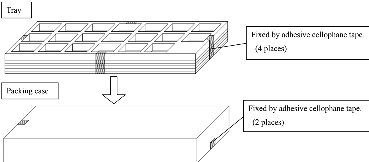
Fig.12 Packing Method
