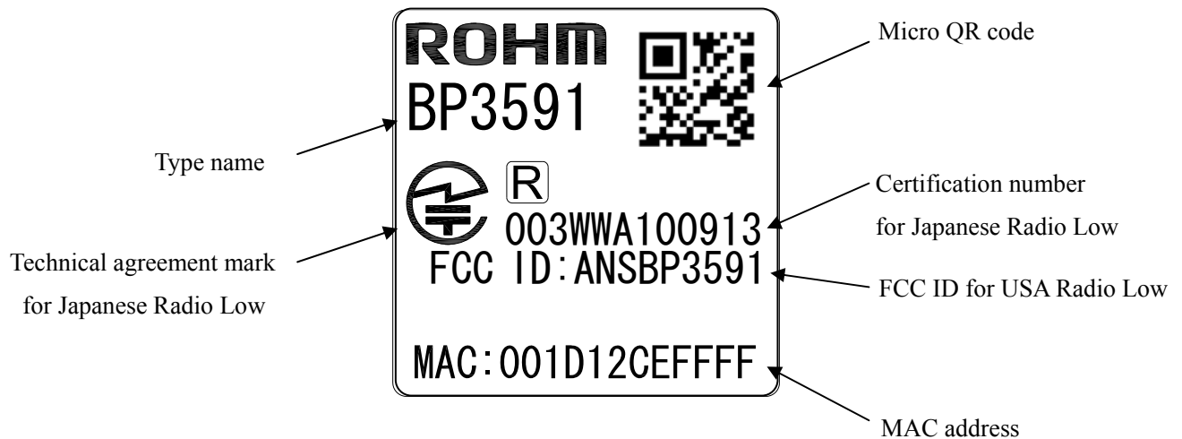
Fig.6 Product Label Spec
