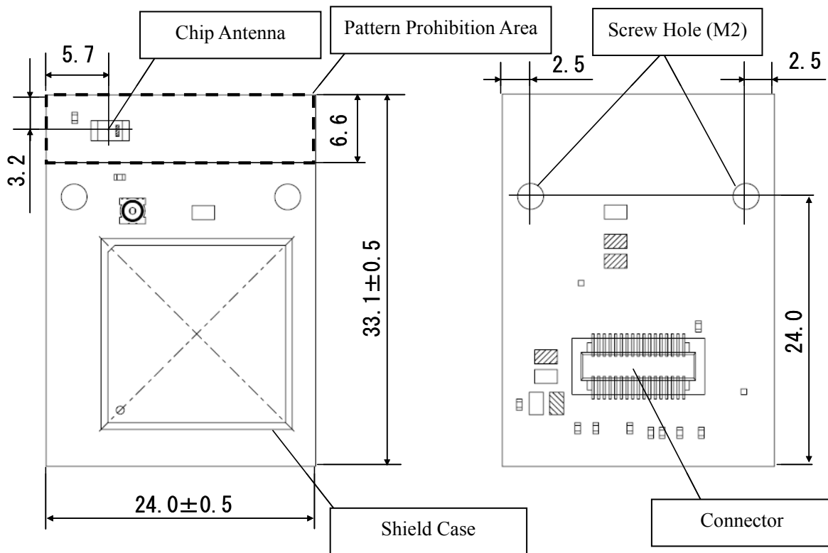
Fig.4 Precautions for Mounting (Unit : mm)
