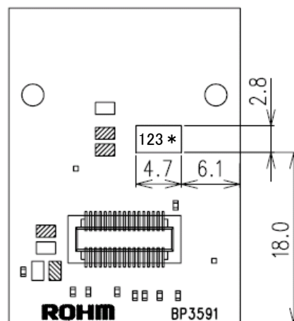
Fig.3 Marking PCB SPEC (Unit: mm)
