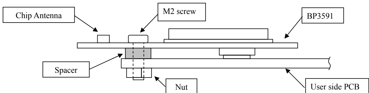
Fig.5 Fixed Module Figure (Side view)
