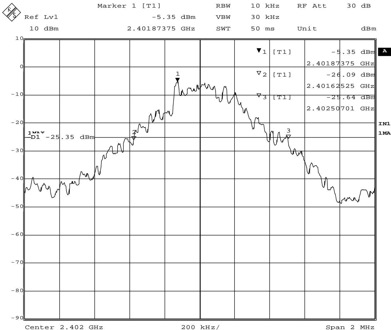
20 dB Bandwidth (TX on 2402MHz)
