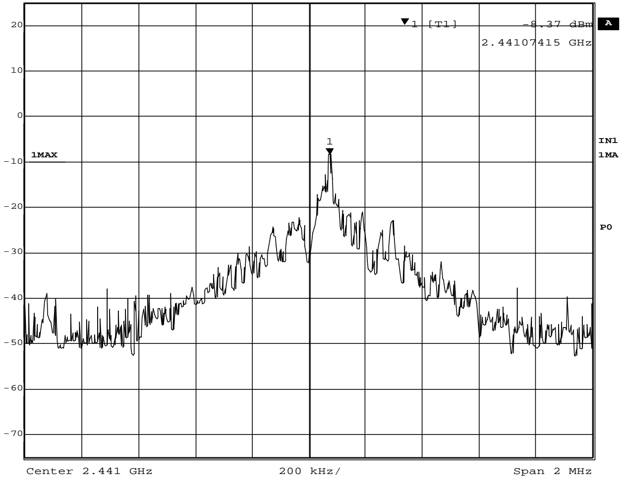
Transmitter Power Spectral Density (Inquiry)
