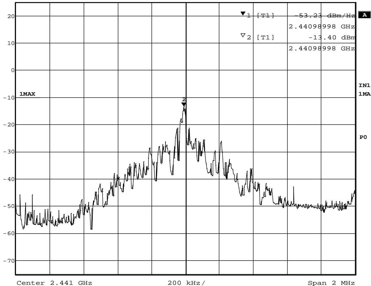
Transmitter Power Spectral Density (Inquiry)
