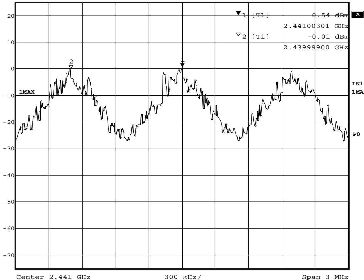
Carrier Frequency Separation
