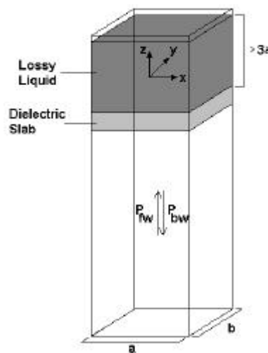
Geometry used for wave-guide calibration (after Ref [2]. Section A.3.2.2)
