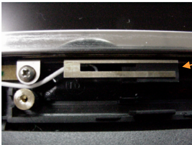
R50 14/15 inch Bluetooth Antenna (Meander Antenna) P/N: 91P6817
