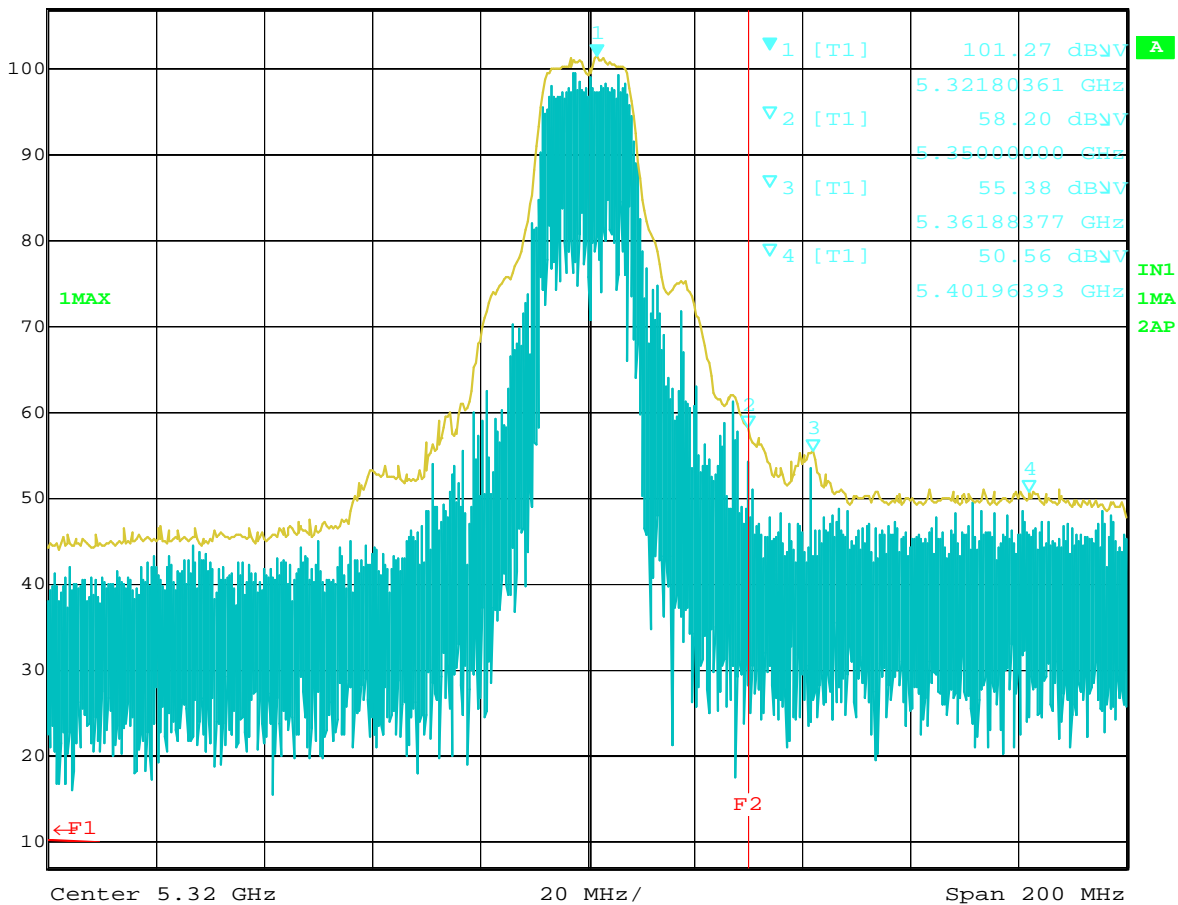
Plot-2-1 Ch.64 5320MHz TX, OFDM 9Mbps (Peak) in "Notebook" operation mode
