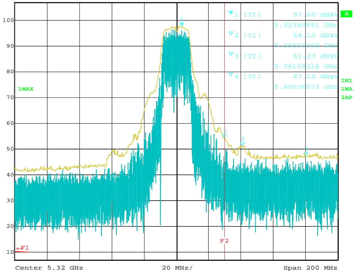
Plot-2-3 Ch.64 5320MHz TX, OFDM 9Mbps (Peak) in "Tablet" operation mode
