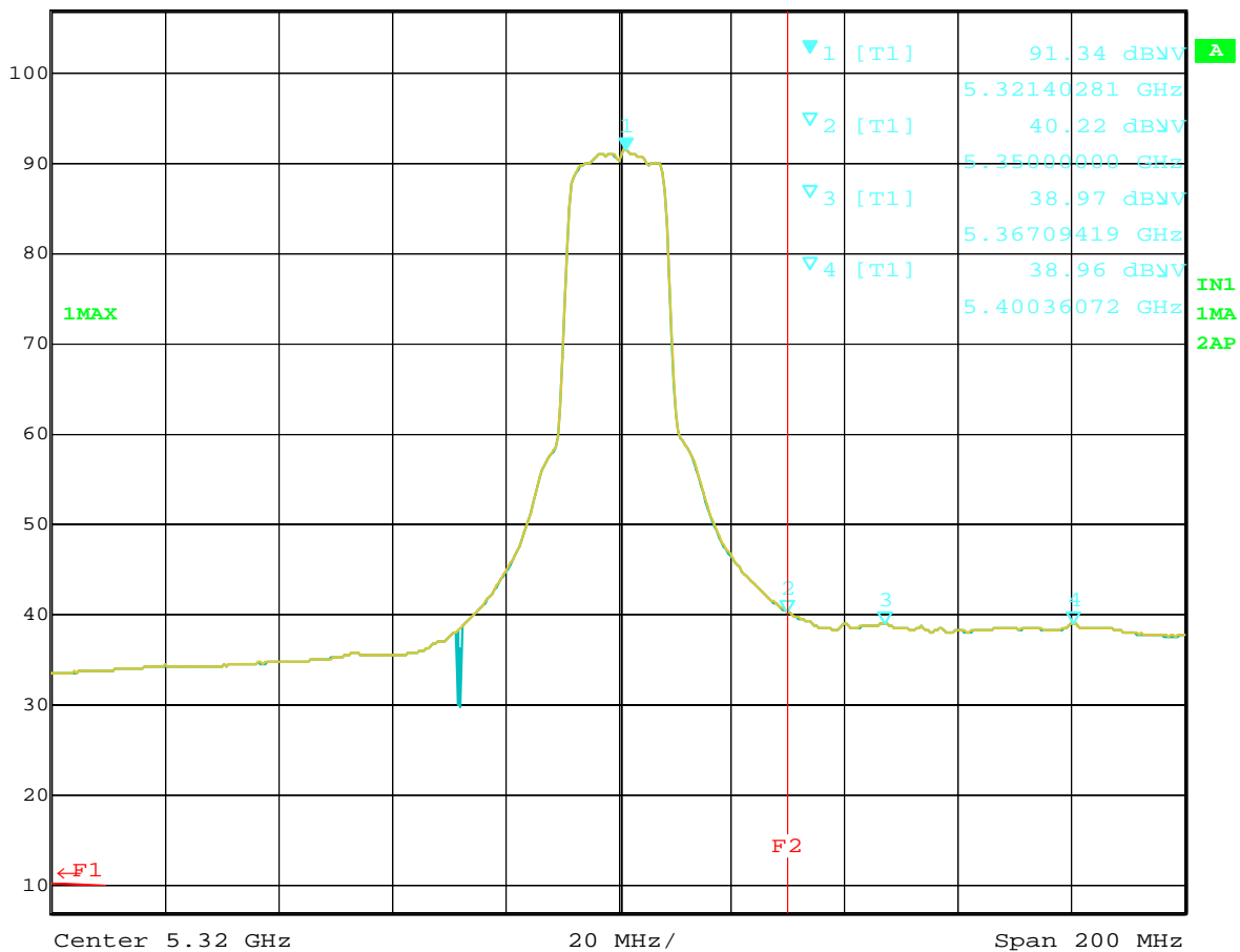
Plot-2-2 Ch.64 5320MHz TX, OFDM 9Mbps (Average) in "Notebook" operation mode
