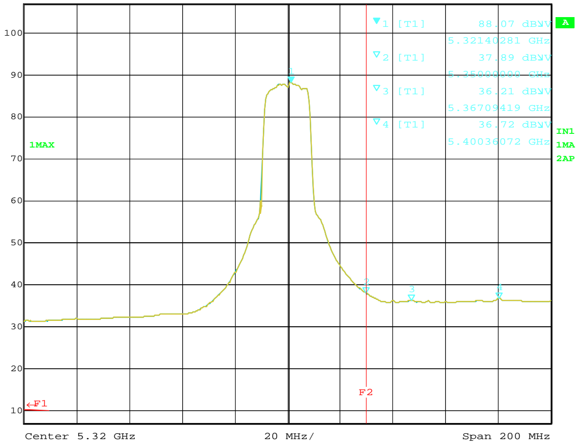
Plot-2-4 Ch.64 5320MHz TX, OFDM 9Mbps (Average) in "Tablet" operation mode
