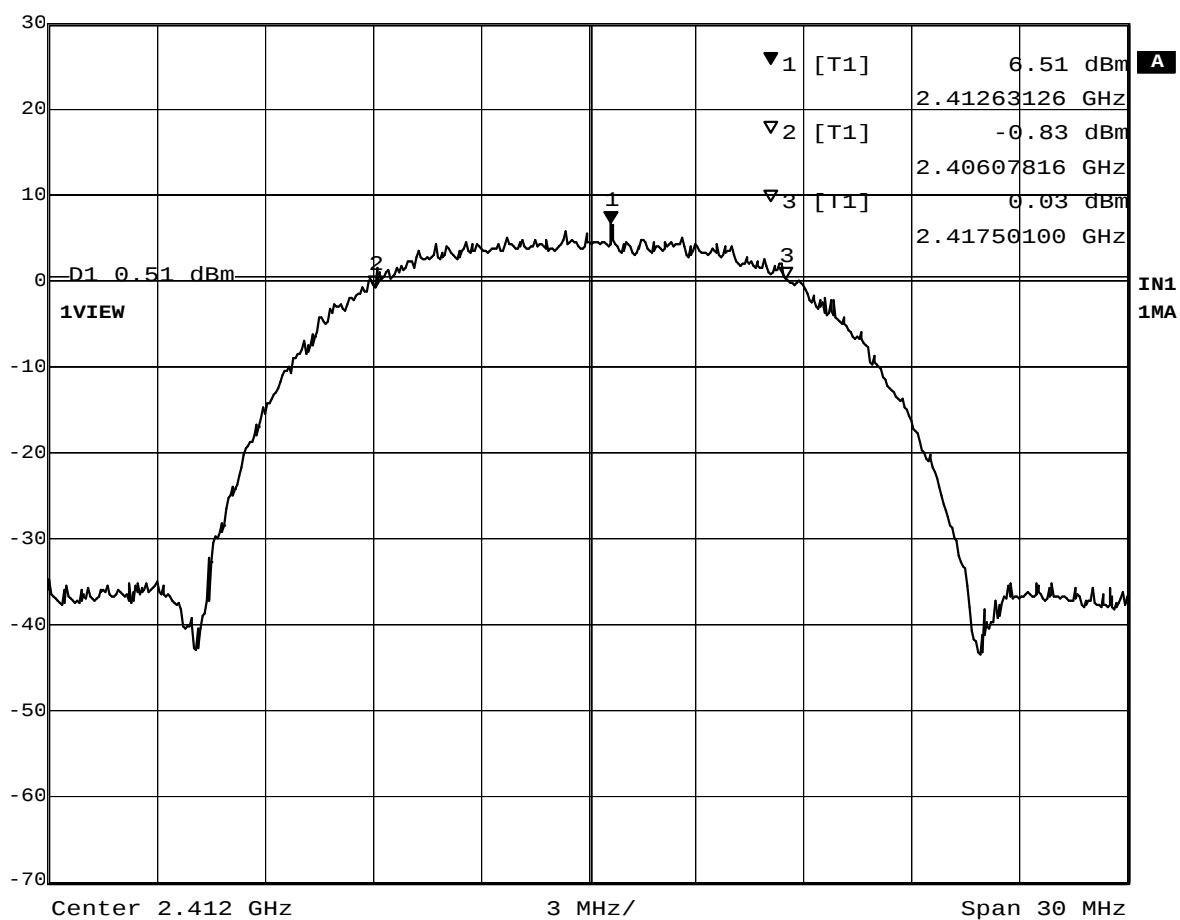
Plot 1-2. 6dB BW at 2412MHz (DSSS, 11Mbps)
