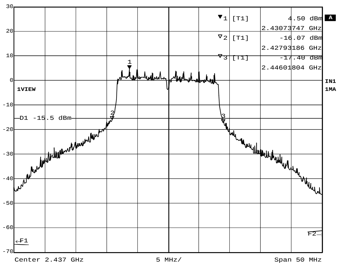
Plot 2-2. 20dB BW at 2437MHz (OFDM, 18Mbps)
