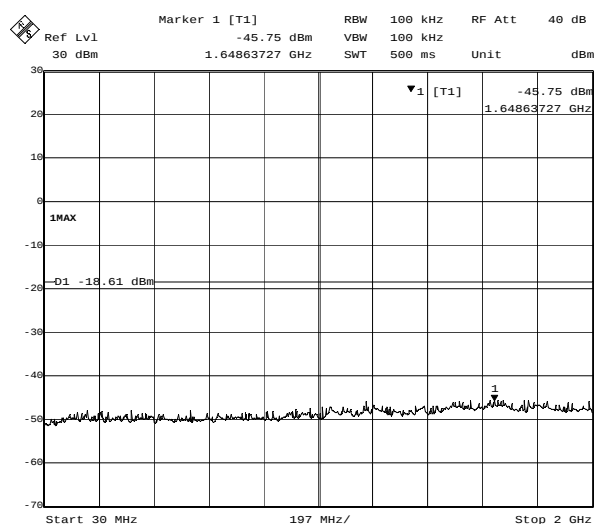
Plot 4-4. Out of band emissions around 2412MHz (OFDM, 18Mbps)
