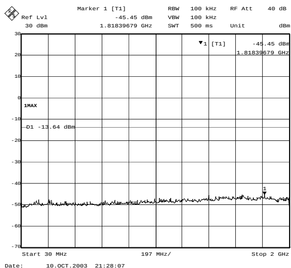
Plot 4-1. Out of band emissions around 2412MHz (DSSS, 11Mbps)
