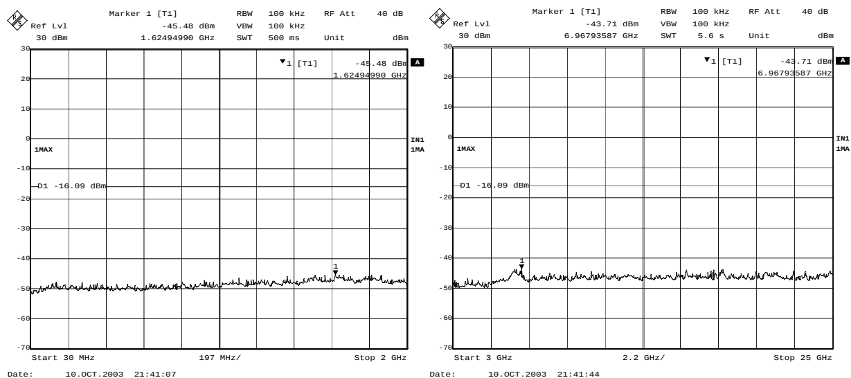
Plot 4-5. Out of band emissions around 2437MHz (OFDM, 18Mbps)
