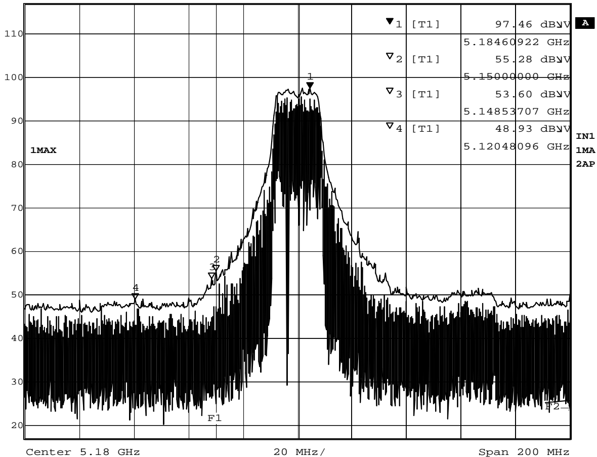
Plot 7-1-1 5180MHz TX mode (Peak)
