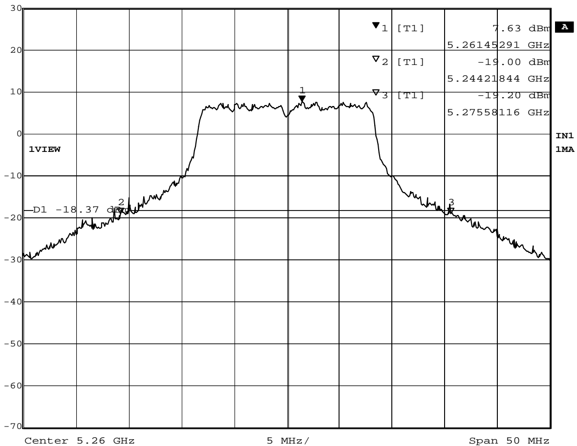
Plot 1-2. 26dB BW at 5260MHz
