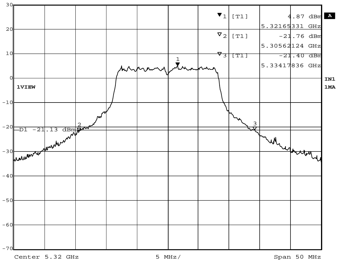
Plot 1-3. 26dB BW at 5320MHz
