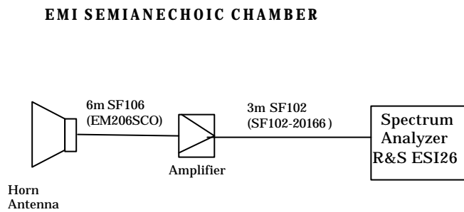
Figure 7-2. Cables for Radiated Emission Test (12.4 - 18GHz)
