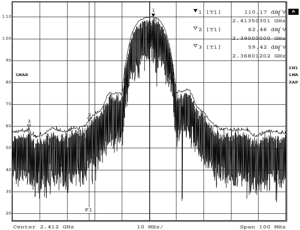
Plot 7-3-1 Ch.1 2412MHz TX 11Mb/s (Peak)
