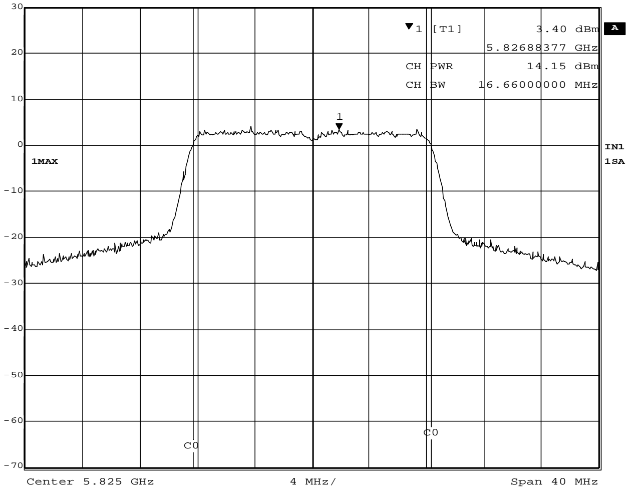
Plot 3-6. Conducted Peak Output Power of 5825MHz
