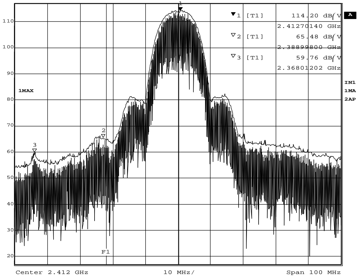
Plot 7-3-1 Ch.1 2412MHz TX 11Mb/s (Peak)
