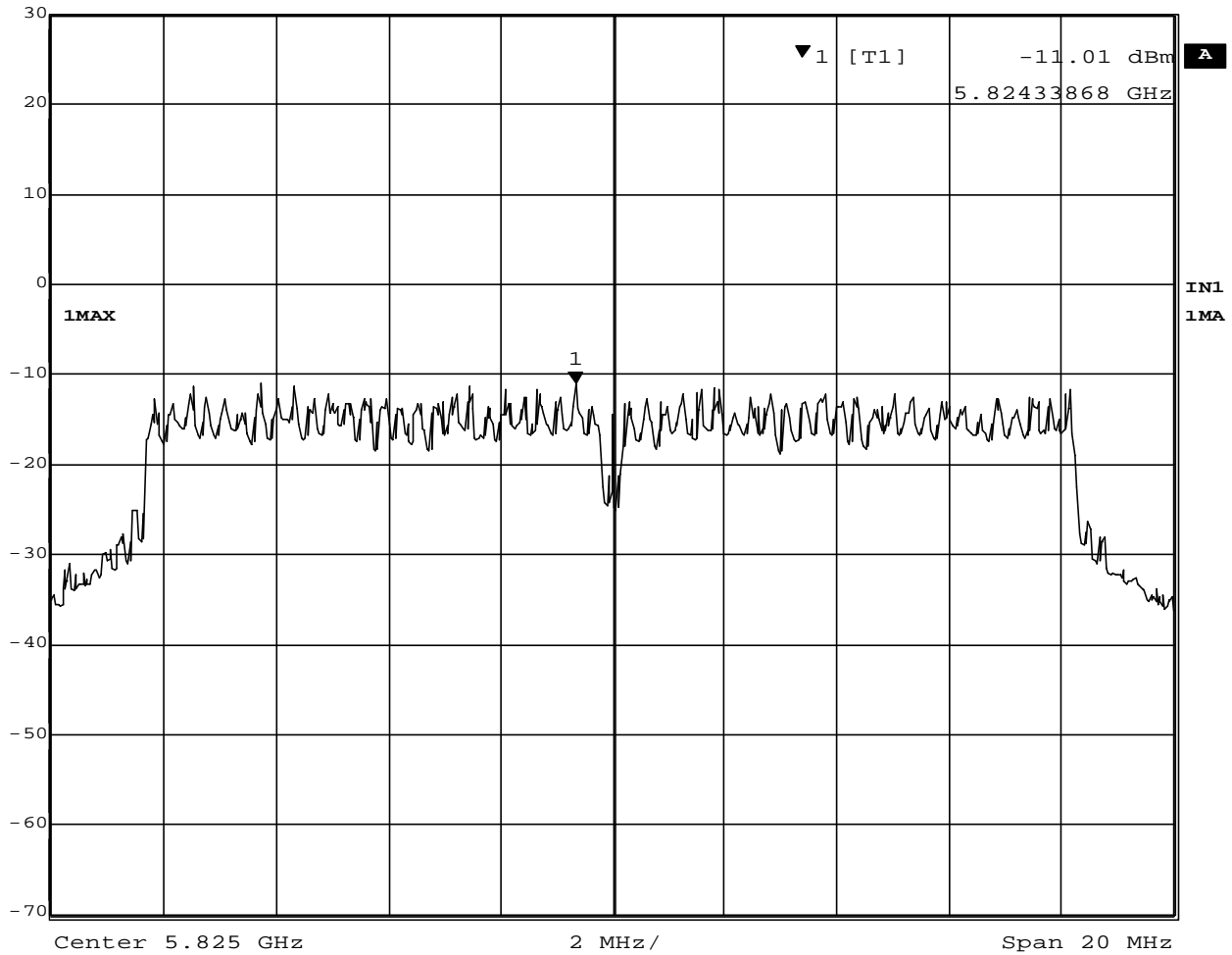
Plot 4-6. Peak Power Spectral Density of 5825MHz
