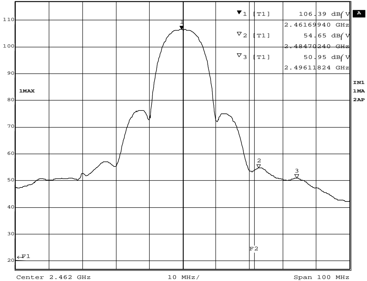
Plot 7-3-4 Ch.1 2462MHz TX 11Mb/s (Average)
