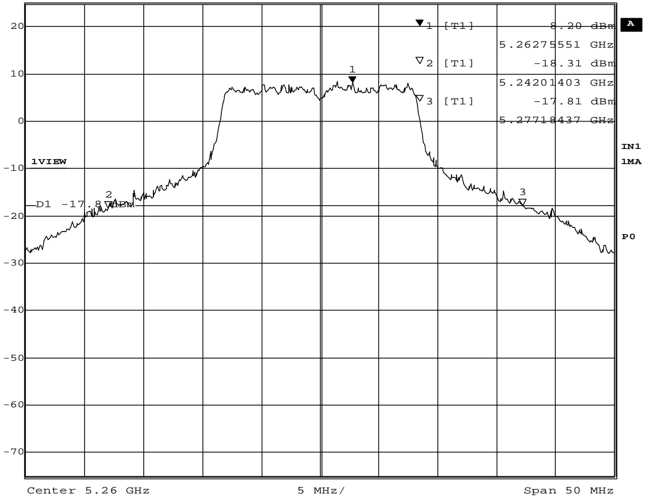
Plot 1-2. 26dB BW at 5260MHz
