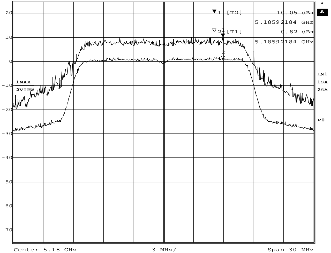
Plot 4-1 Peak Excursion Ratio at 5180MHz
