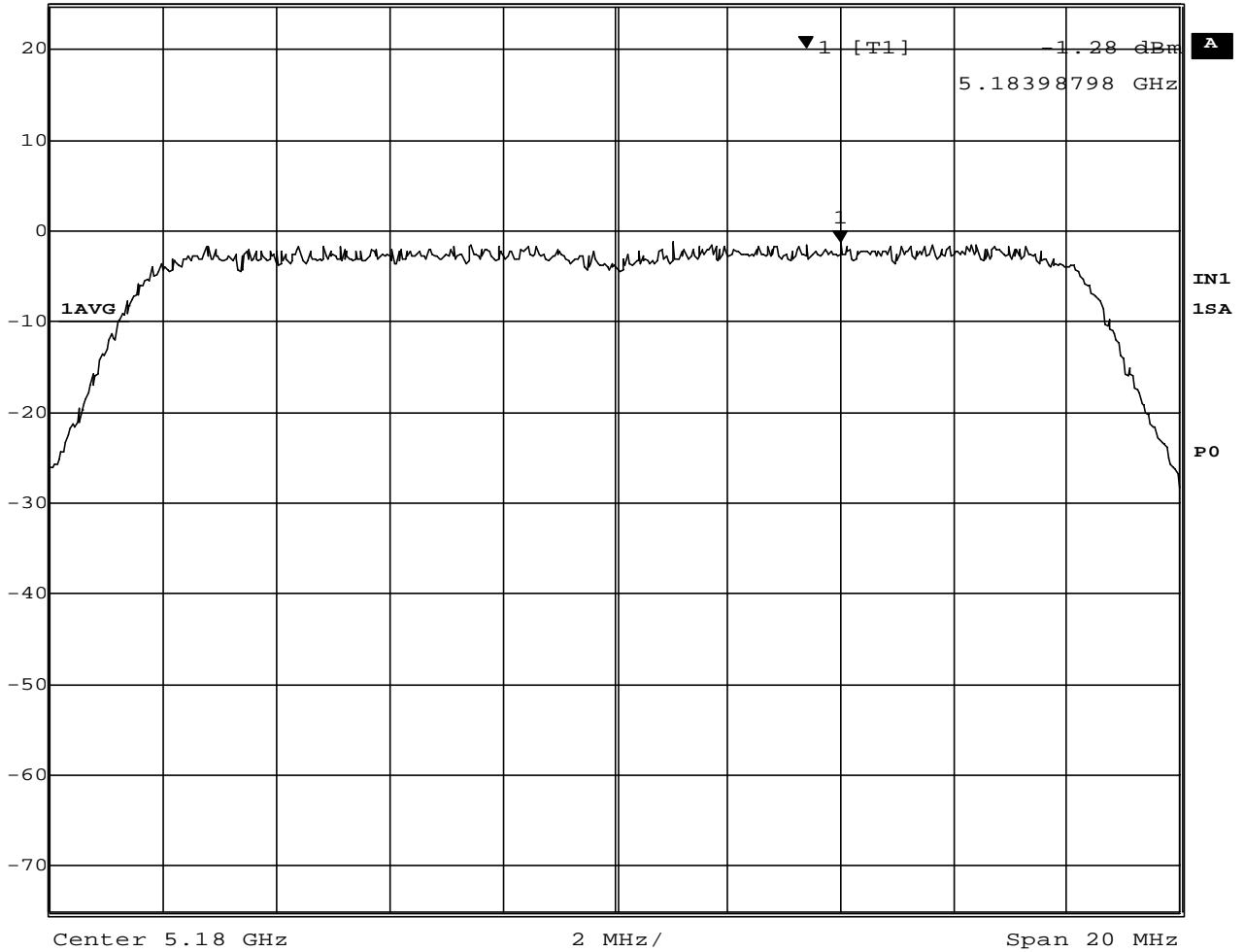
Plot 3-1 Peak Power Spectral Density at 5180MHz
