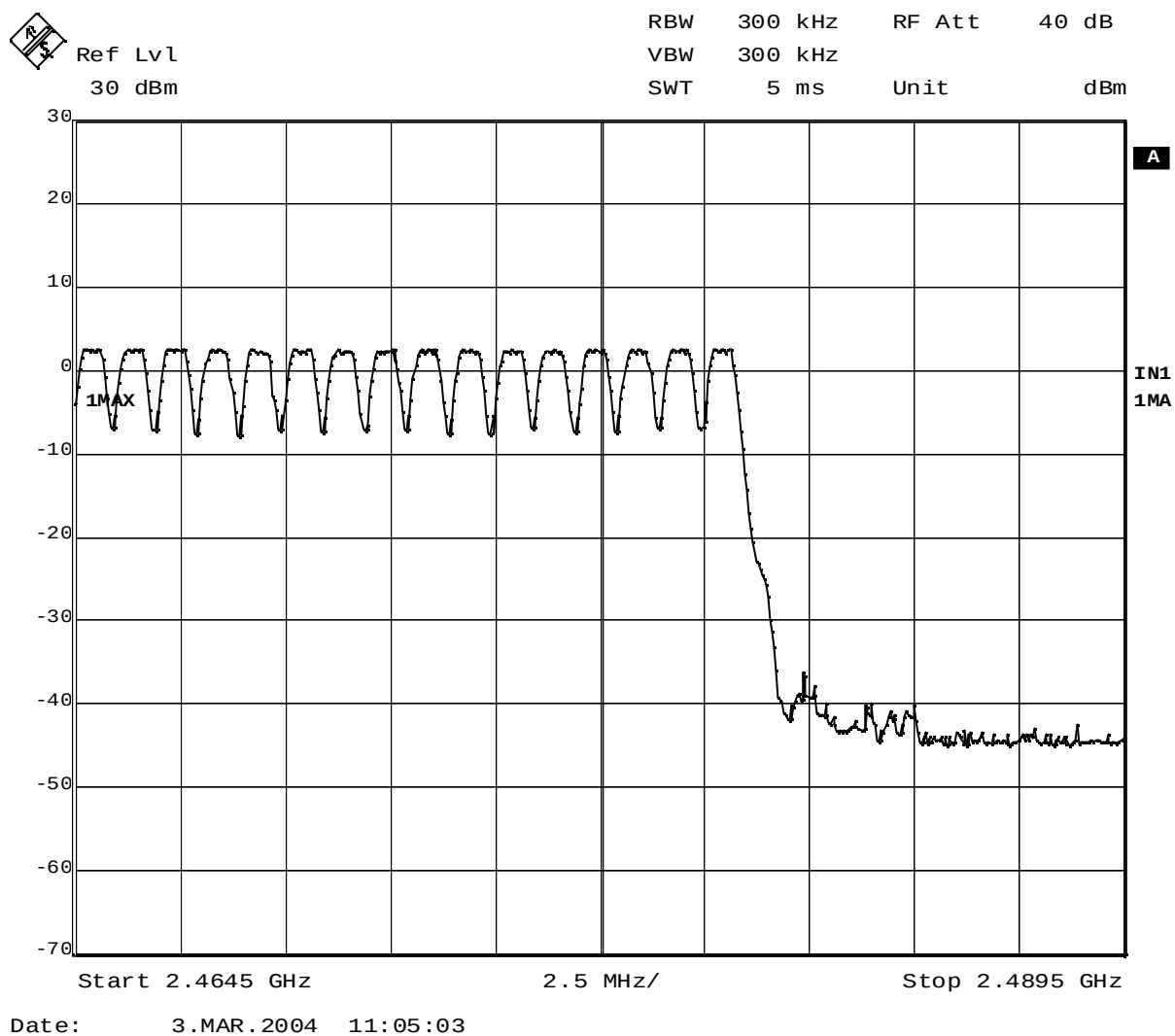
Plot 2-4. Number of Hopping Frequencies (range 4)
