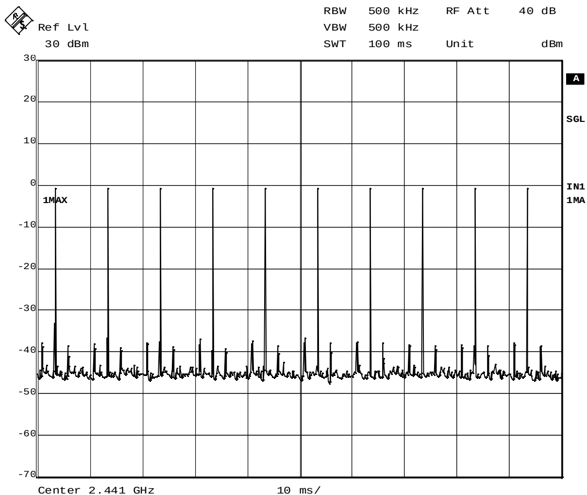
Plot 4-2. Time of Occupancy (Inquiry, Repetition rate)
