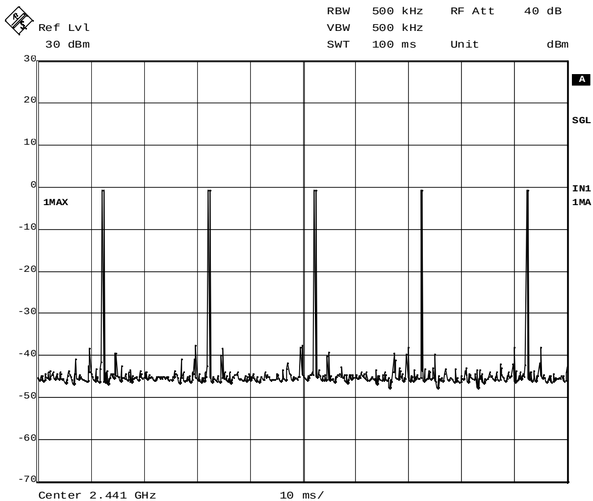
Plot 4-4. Time of Occupancy (Paging, Repetition rate)
