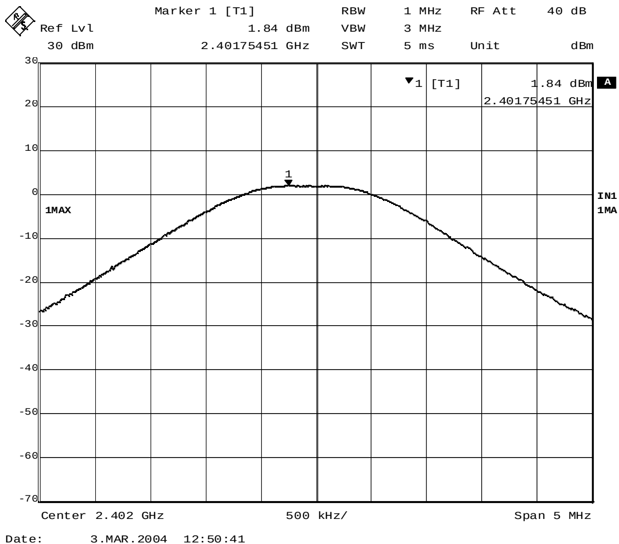
Plot 5-1. Peak Output Power (TX on 2402MHz)
