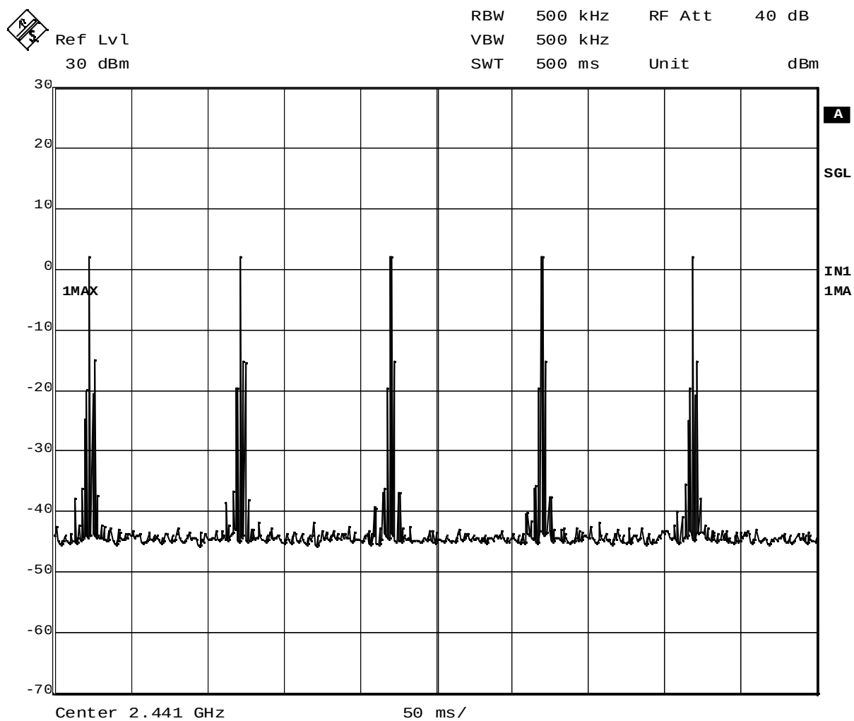
Plot 4-6. Time of Occupancy (Data transmission, Repetition rate)
