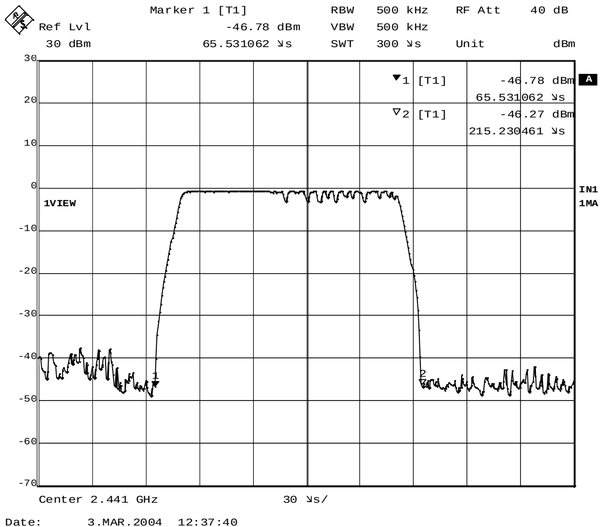
Plot 4-1. Time of Occupancy (Inquiry, Burst duration)
