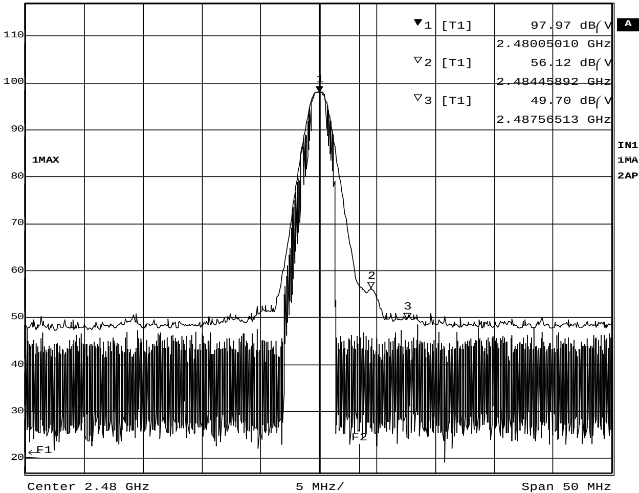
Plot 11-2-3 Ch.79 2480MHz TX (Peak)
