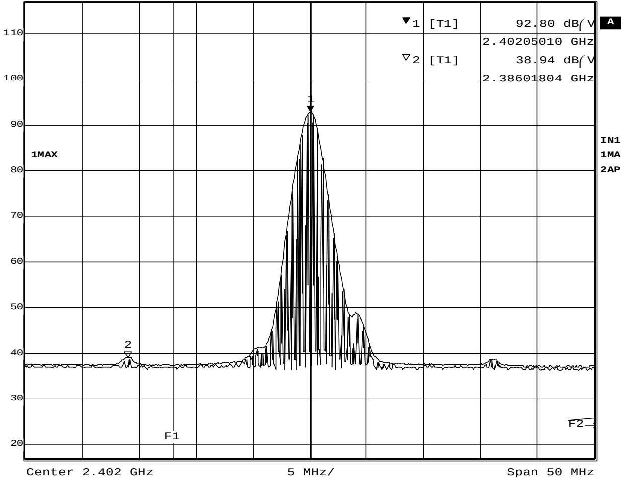
Plot 11-2-2 Ch.1 2402MHz TX (Average)
