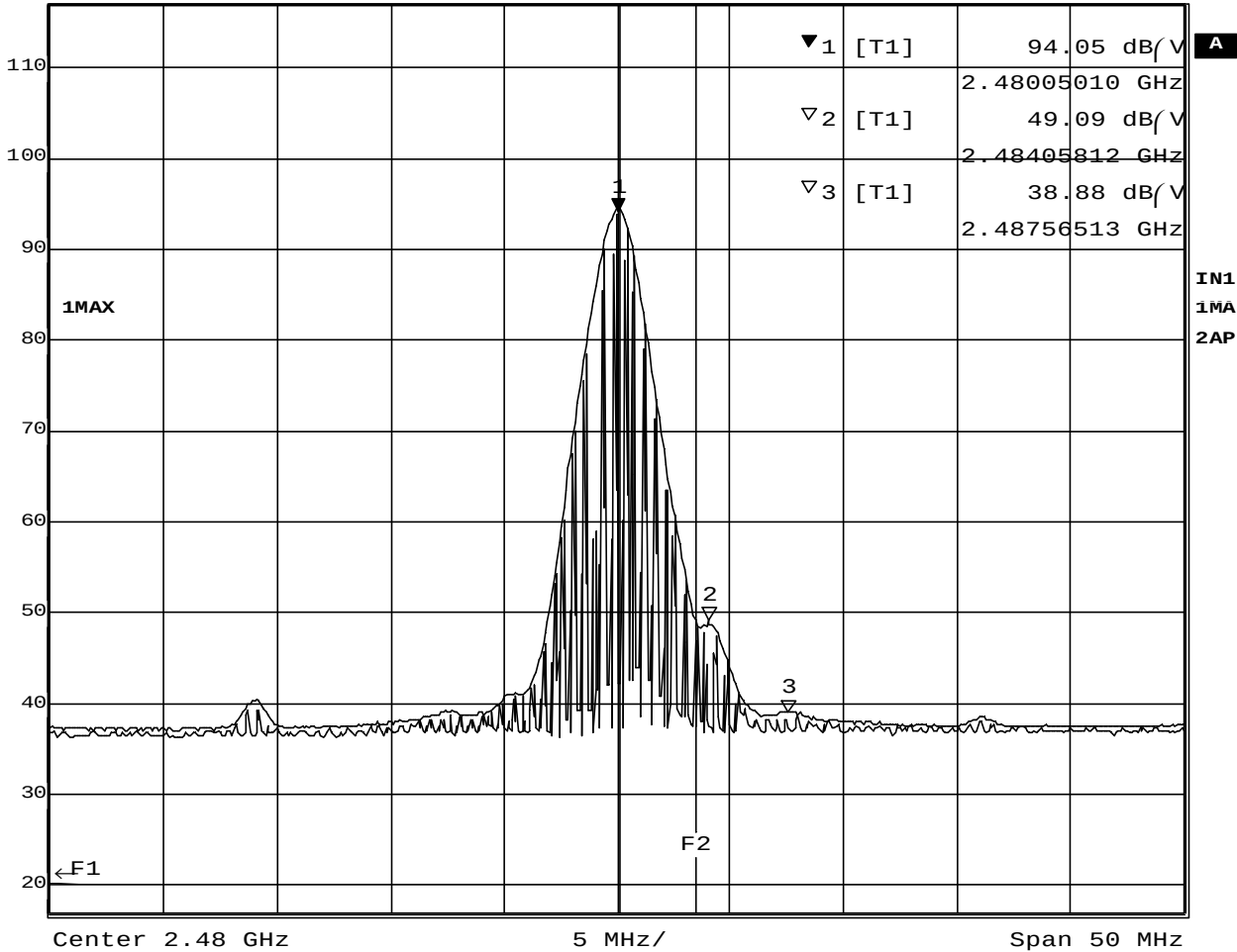
Plot 11-2-4 Ch.79 2480MHz TX (Average)
