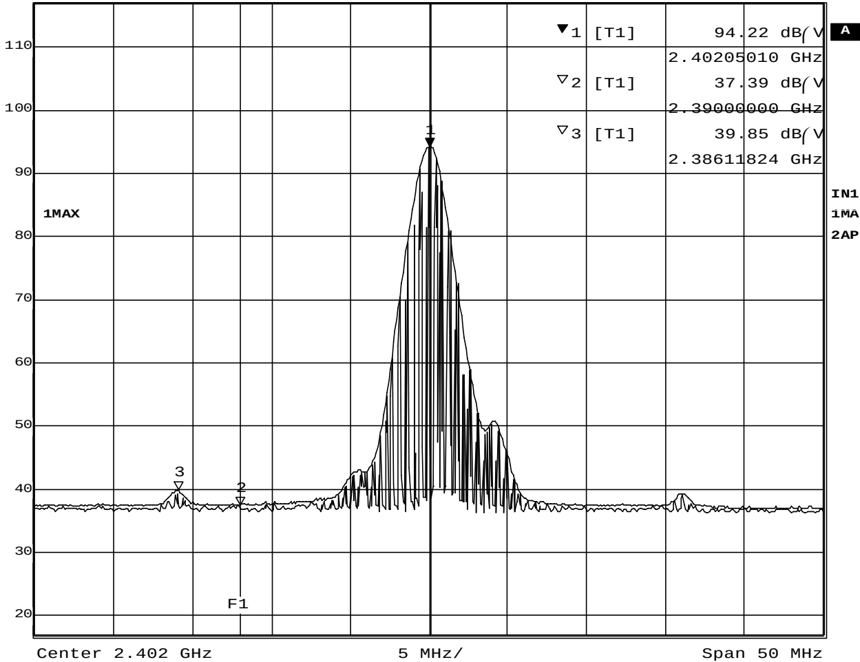
Plot 11-2-2 Ch.1 2402MHz TX (Average)
