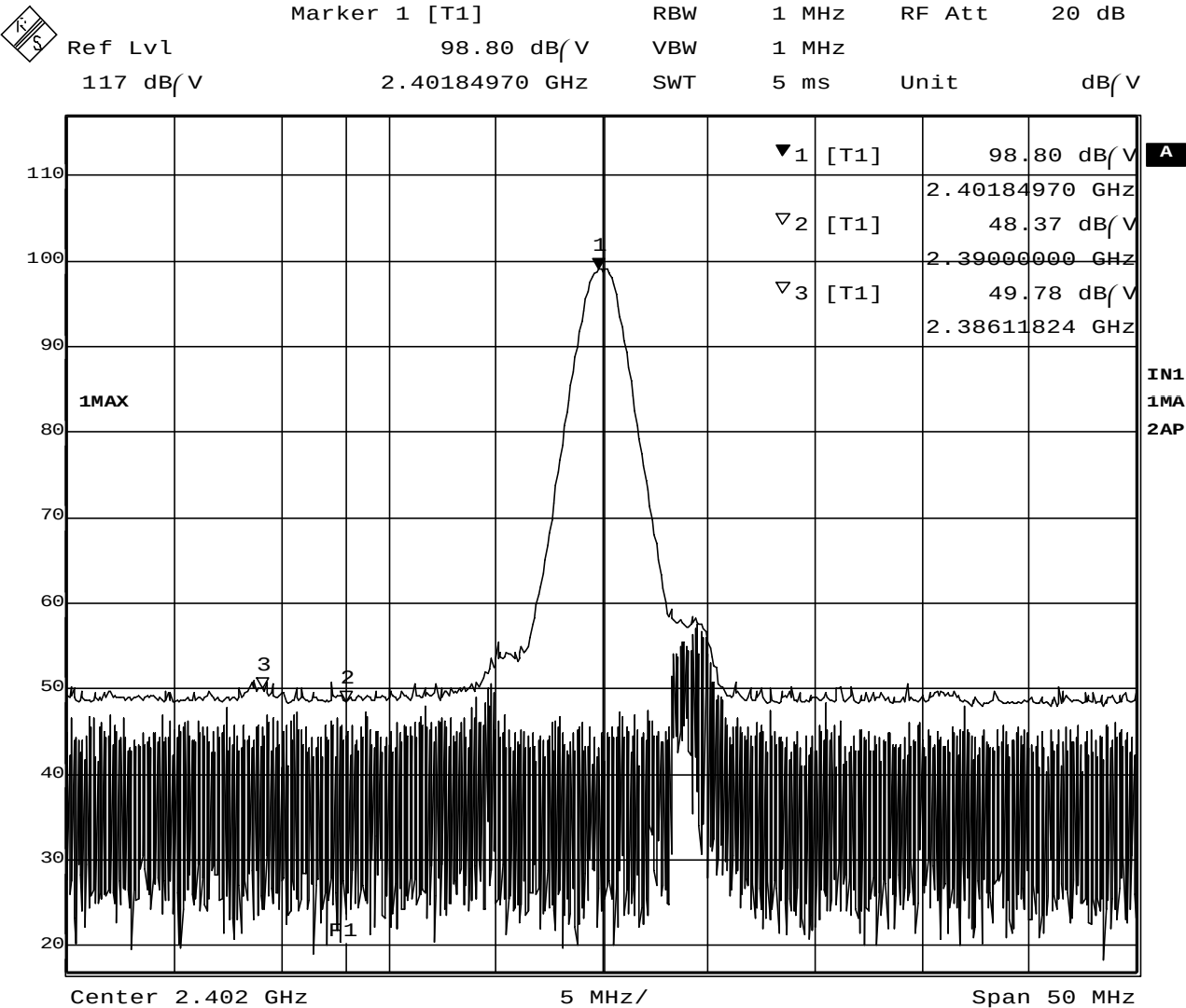
Plot 11-2-1 Ch.1 2402MHz TX (Peak)
