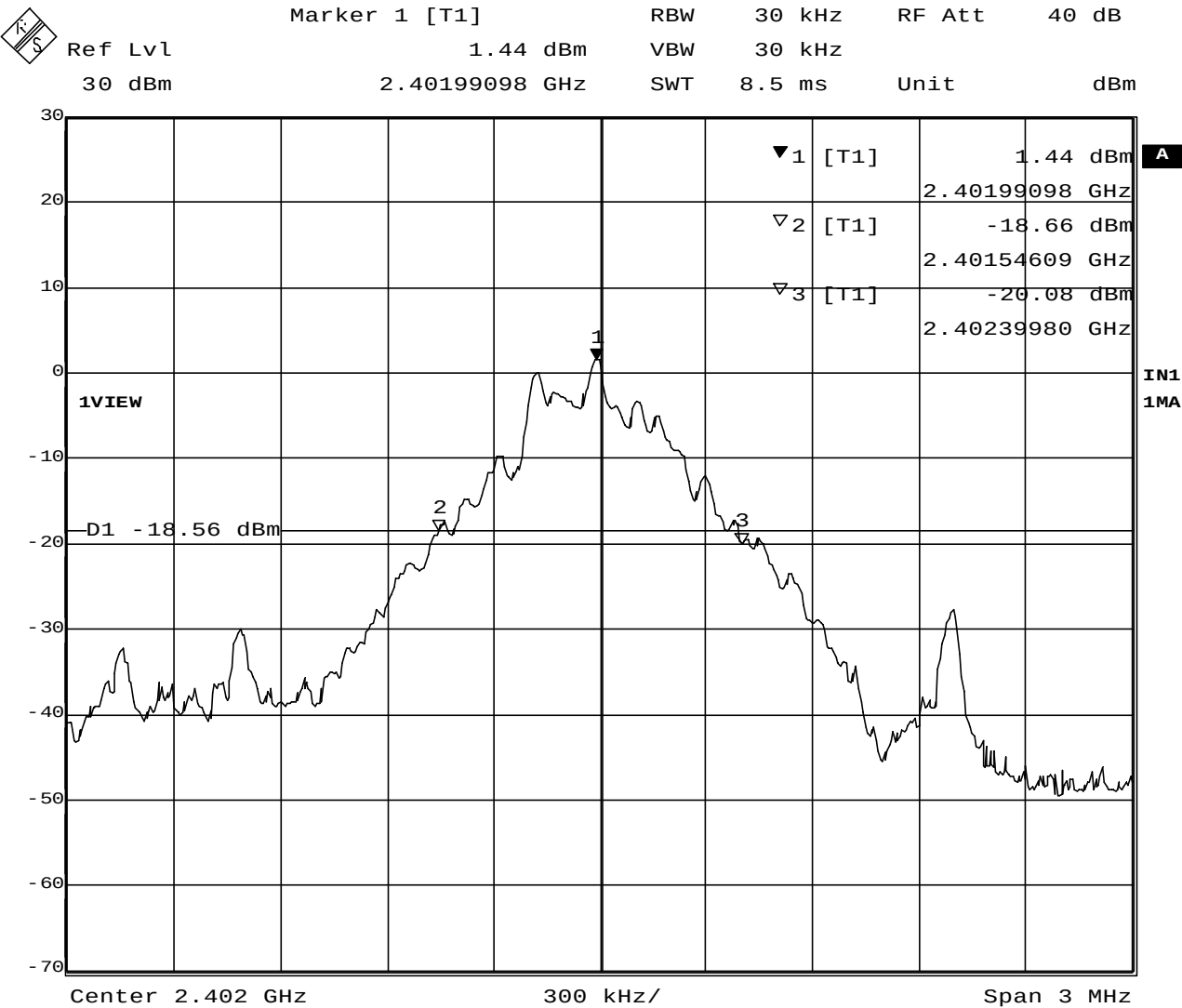
Band-edge (TX on 2402MHz)
