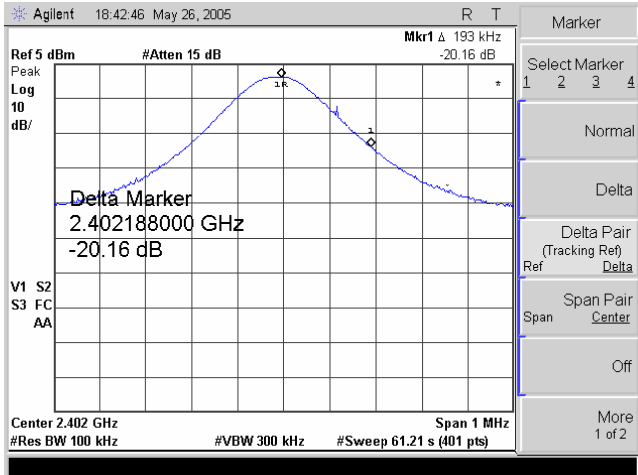
Plot 2. Occupied Bandwidth; Test Results (2.402GHz); F_{HIGH}
