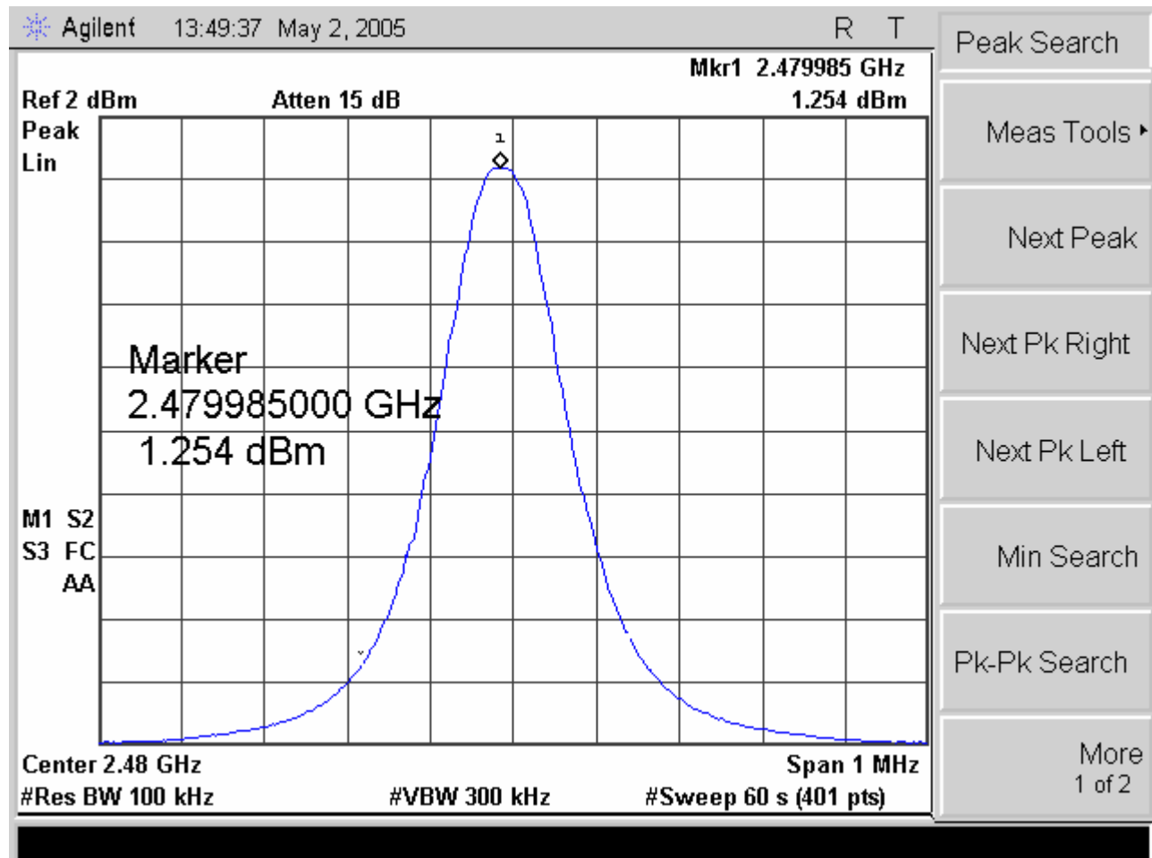
Plot 16. RF Conducted Results –High Channel; Test Results
