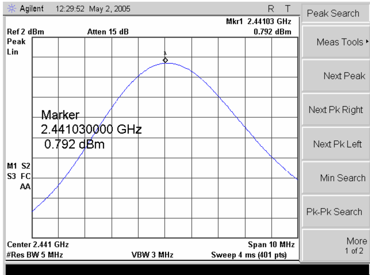
Plot 8. Output Power Test Results
