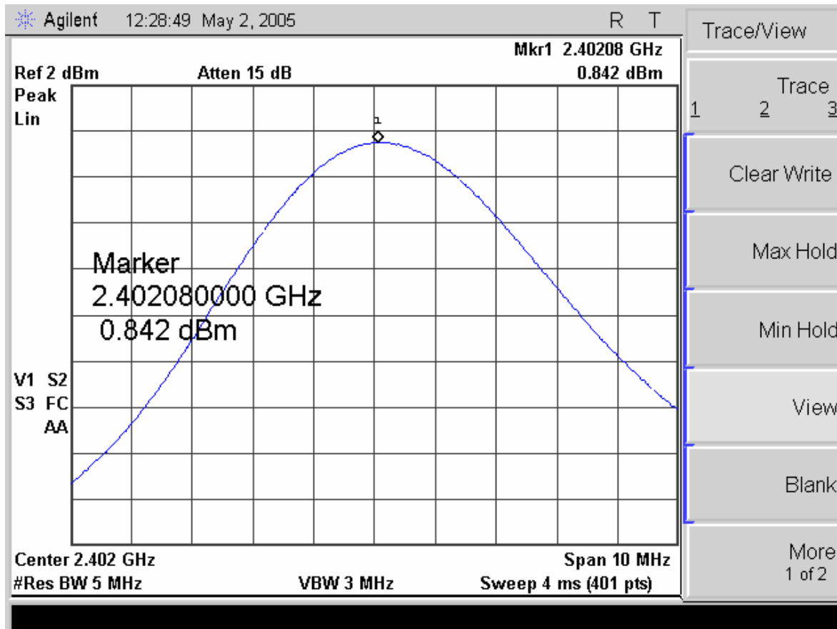
Plot 7. Output Power Test Results
