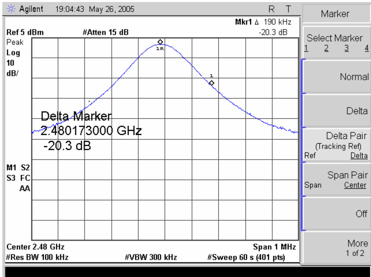
Plot 6. Occupied Bandwidth; Test Results (2.480GHz); F_{\text{HIGH}}
