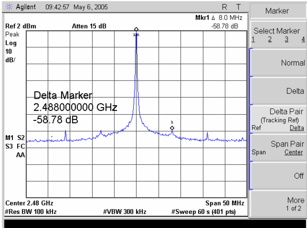
Plot 22. RF Conducted Results – Upper Band Edge
