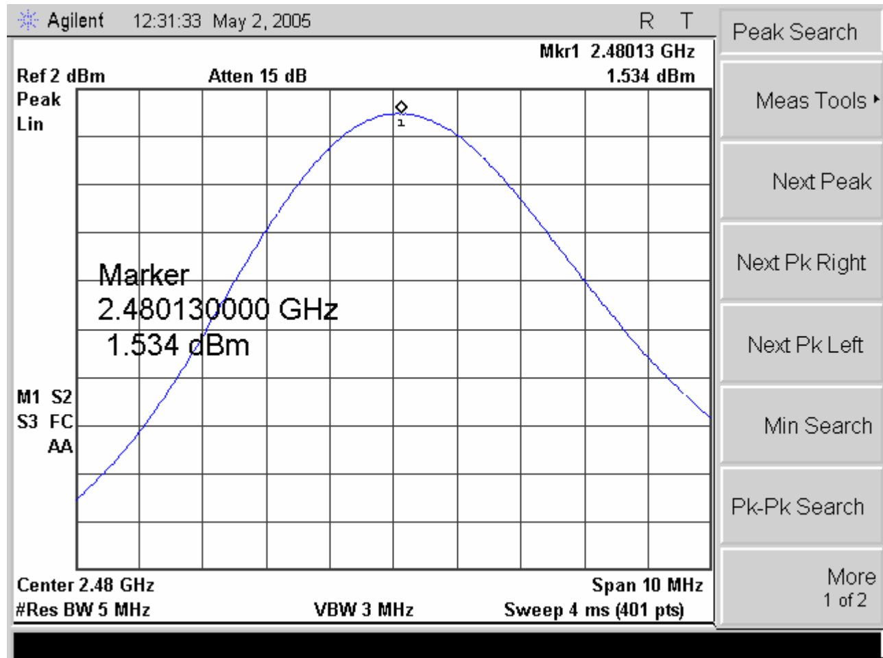
Plot 9. Output Power Test Results
