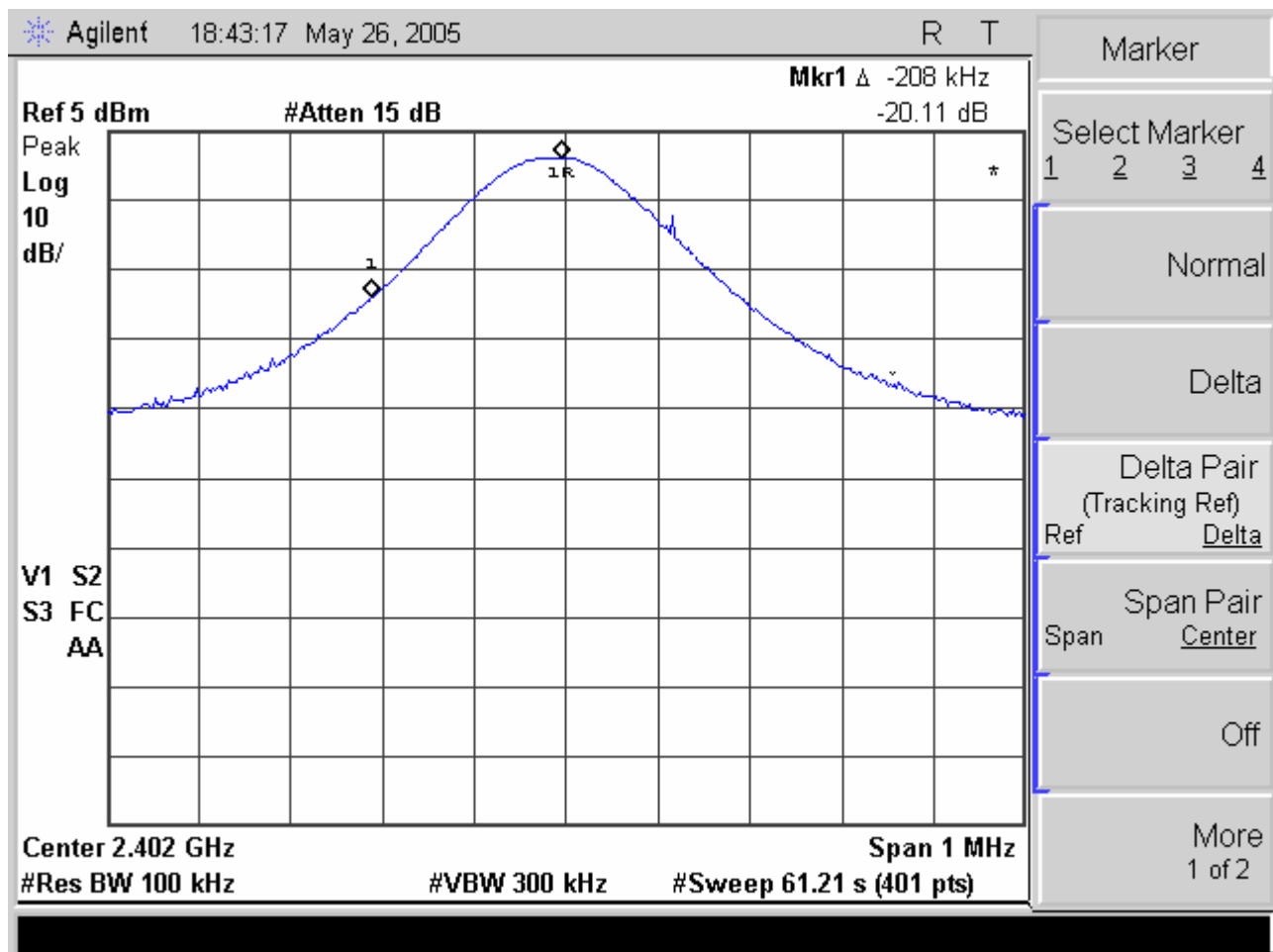
Plot 1. Occupied Bandwidth; Test Results (2.402GHz); F_{Low}
