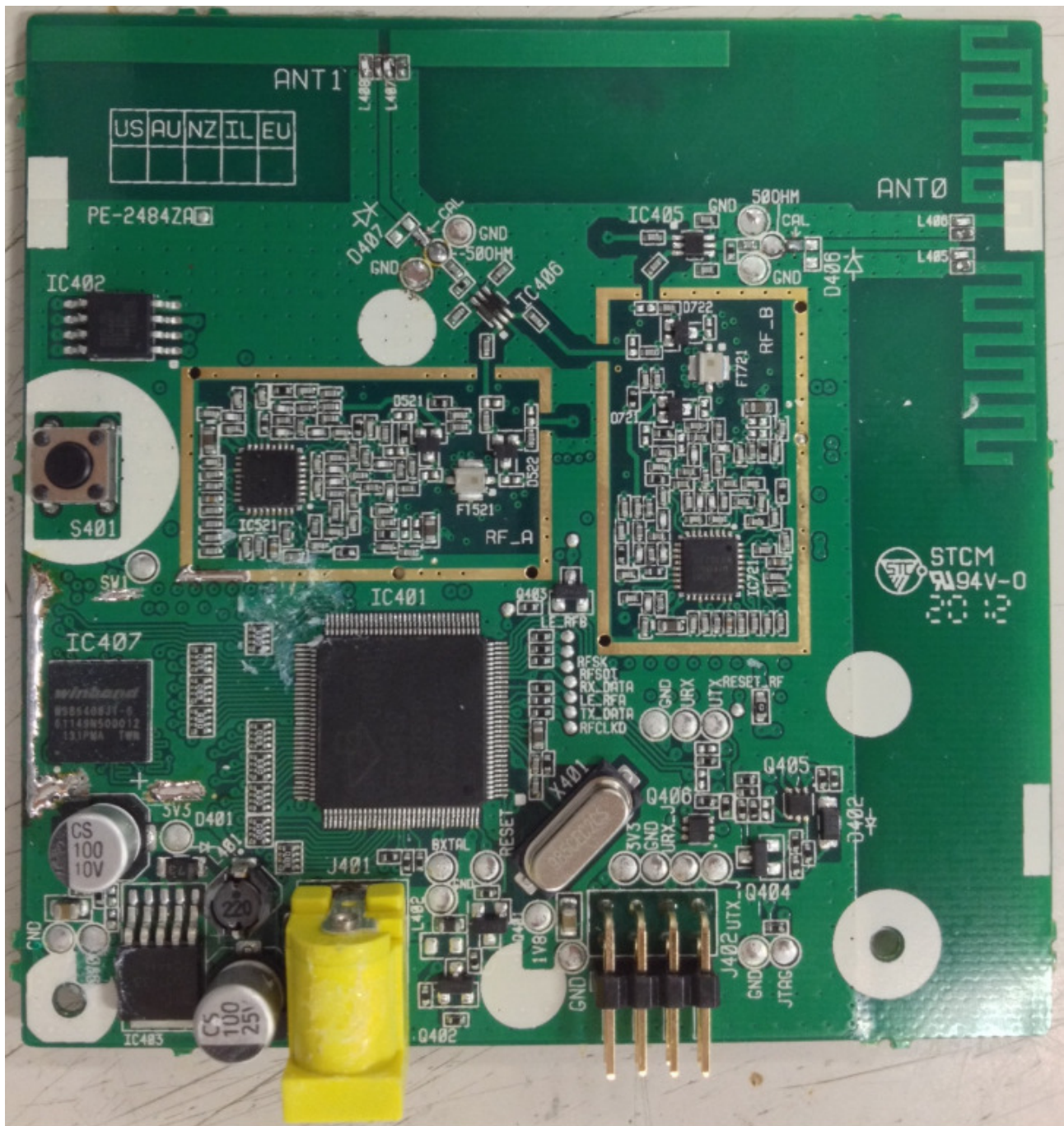
Shield Case Opened [Top view] ( "D100 DECT Repeater NA" )
