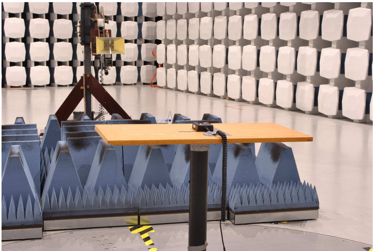
Antenna Gain Measurement
