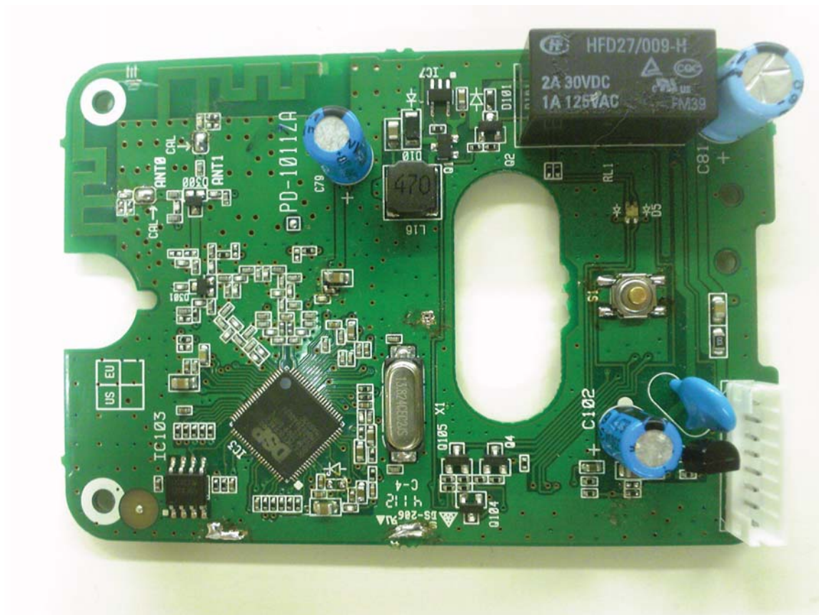
Main PCB Top View - Shield Plate removed
