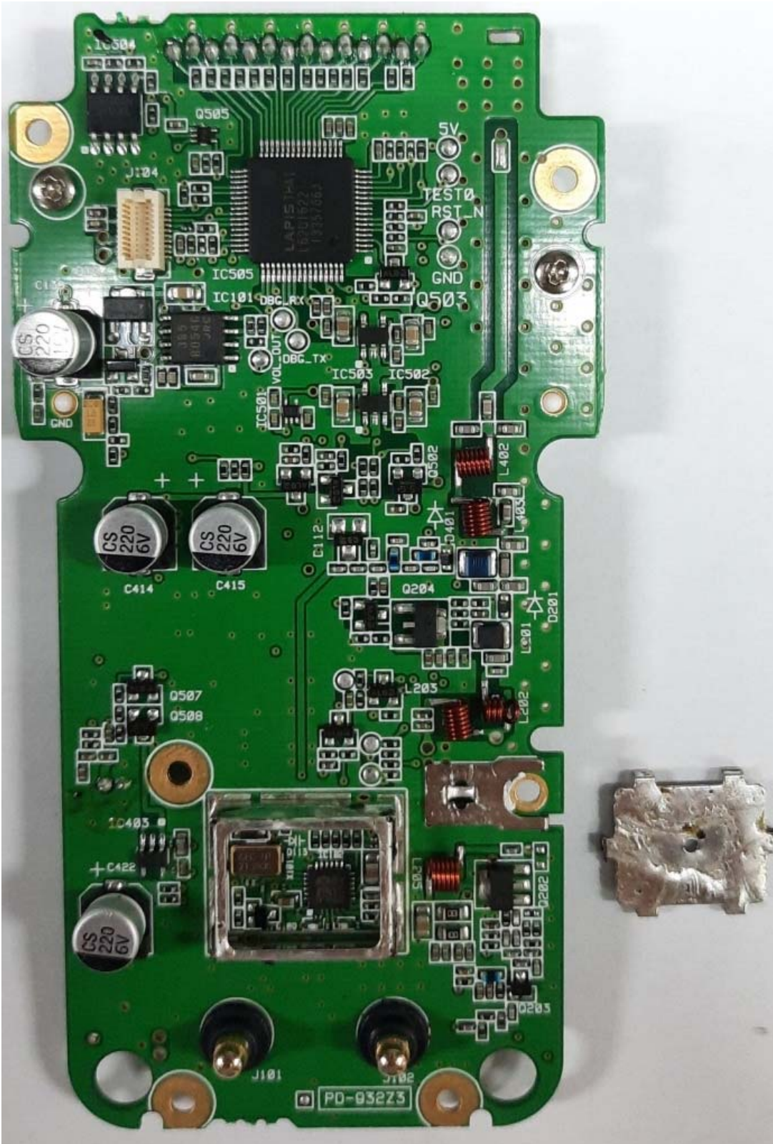
Figure E22.7 – Internal, Main PCB Component Side, Shield Removed
