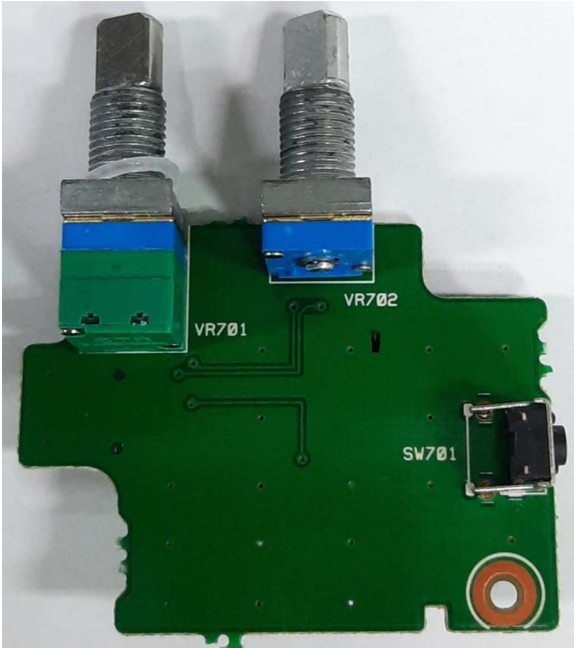
Figure E22.9 – Internal, Interface PCB, Top
