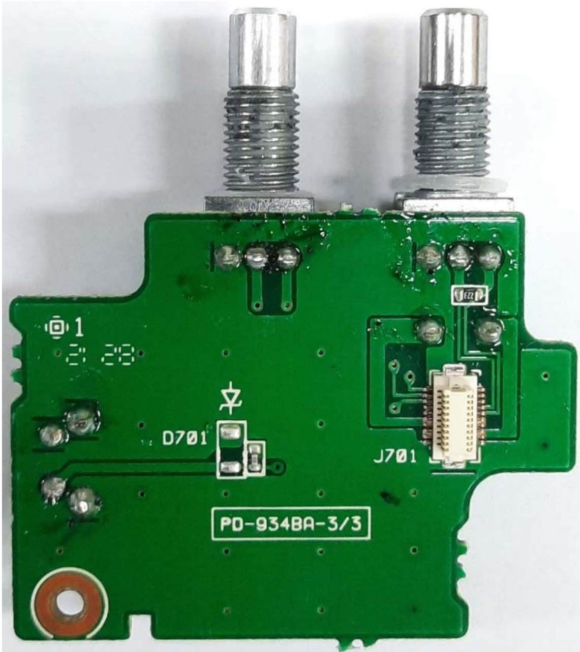
Figure E22.8 – Internal, Interface PCB, Bottom
