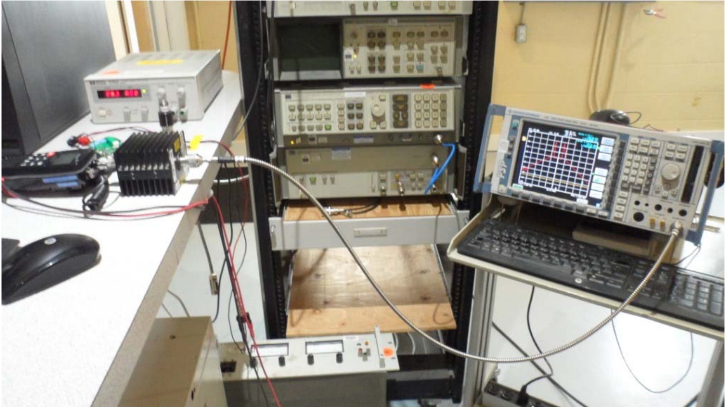
Figure E21.1 – Setup Photo – Conducted Measurements
