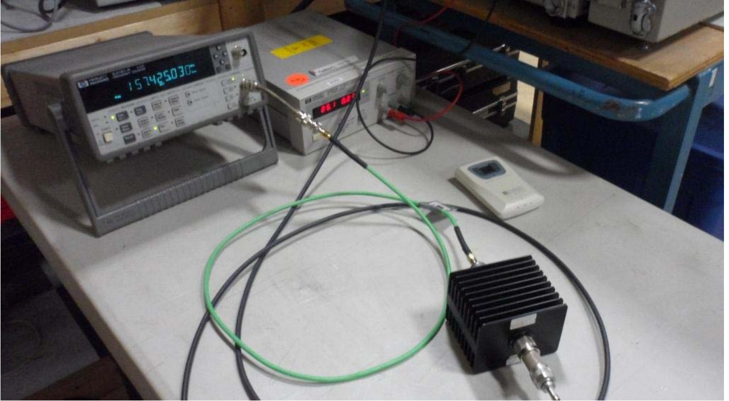
Figure E20.4 – Setup Photo – Frequency Stability Measurements
