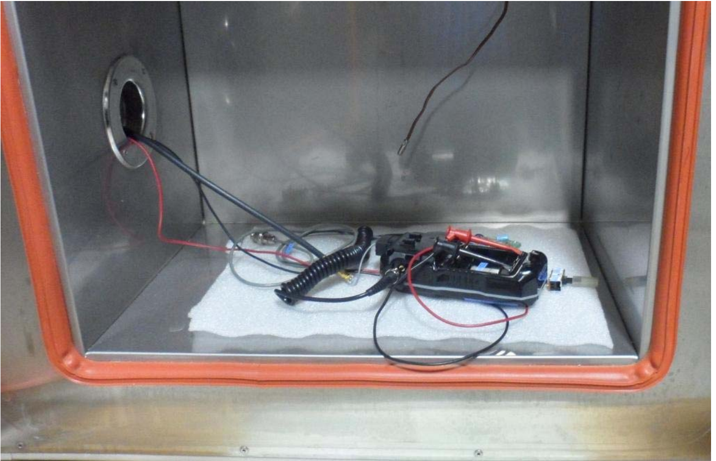
Figure E20.5 – Setup Photo – Frequency Stability Measurements
