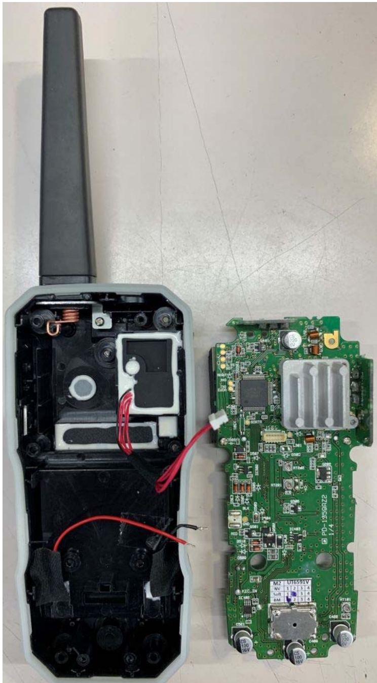
Figure E19.4 – Internal Photo – Main PCB Component Side
