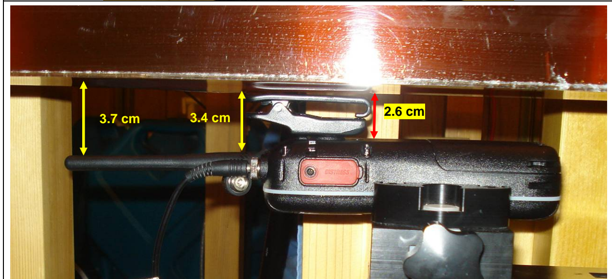
Body-worn Test Setup - DUT with Swivel Belt-clip and Speaker-Microphone accessories
