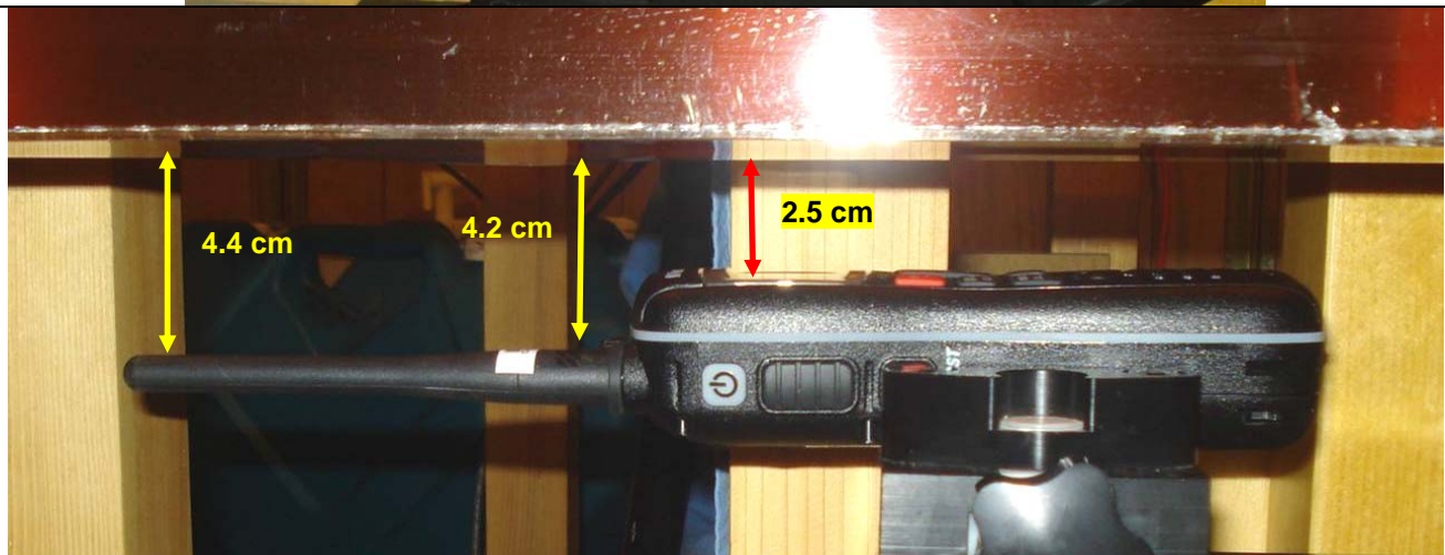
Face-held Test Setup
