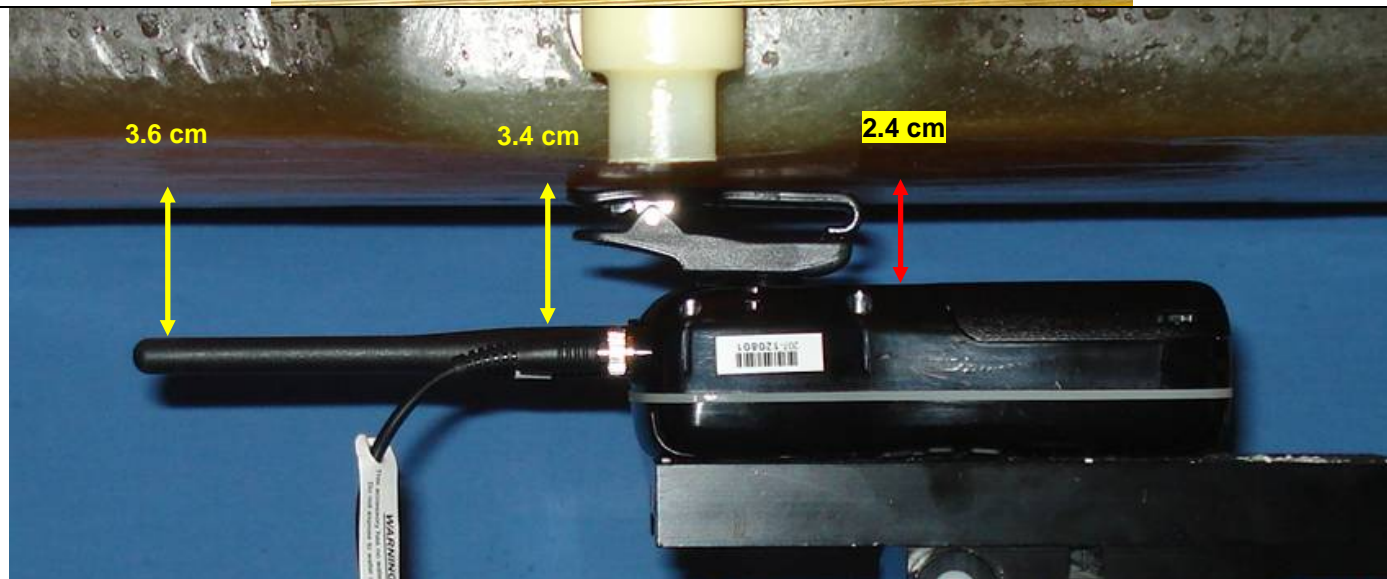
Body-worn Test Setup
