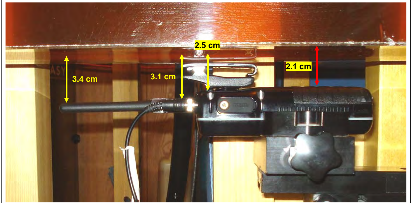
Body-worn Test Setup - DUT with Swivel Belt-clip and Speaker-Microphone accessories
