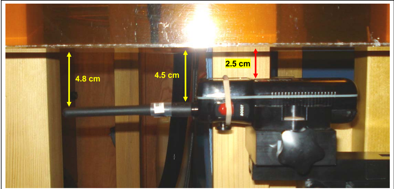
Face-held Test Setup
