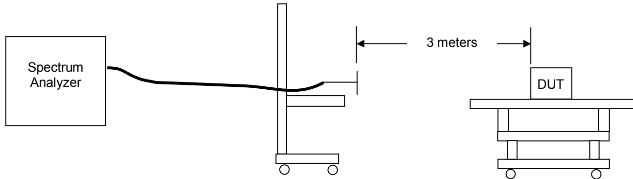
Figure A.5-1 - Setup Drawing – RF Output Power
