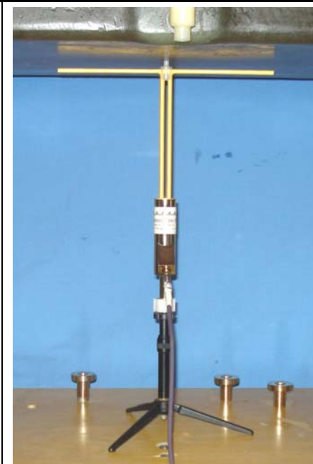
SPEAG 450 MHz Validation Dipole Setup
