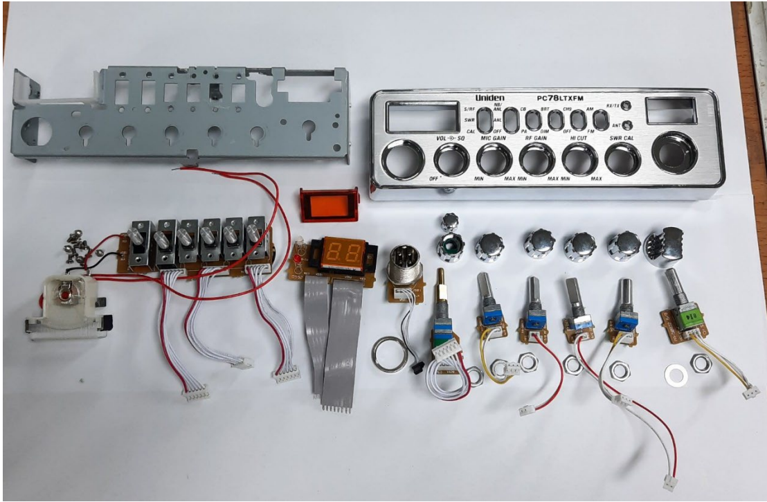
Front Assembly 3
