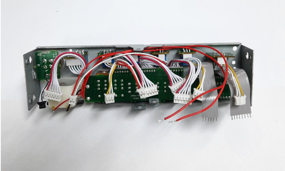
Front Assembly 1
