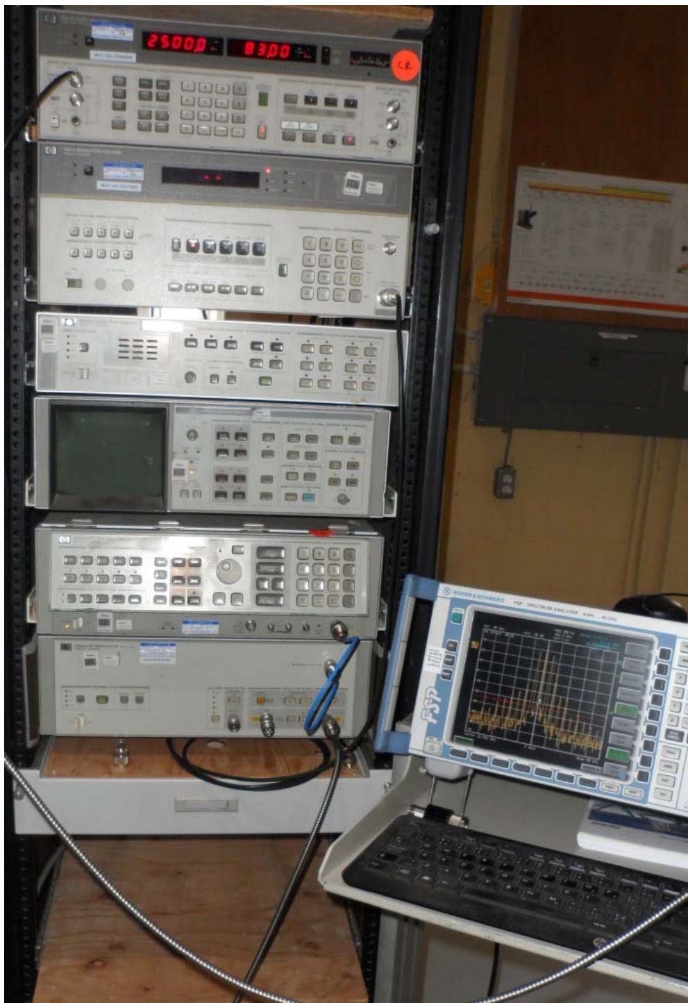
Figure E21.3 – Setup Photo – Occupied Bandwidth
