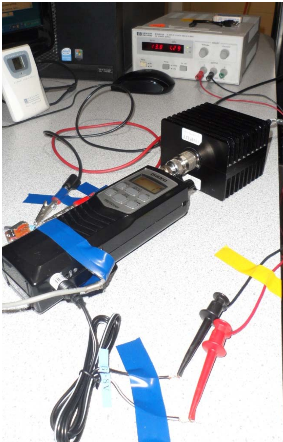
Figure E21.1 – Setup Photo – Conducted Measurements
