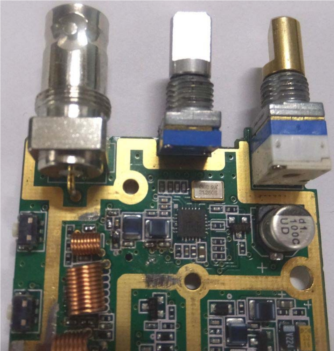
Figure E20.5 – Internal Photo – Main PCB Component Side- Transmit Section
