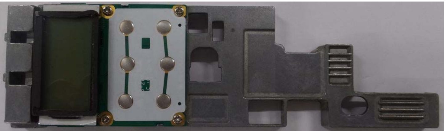
Figure E20.3 – Internal Photo – Front Cover Removed –Display Front Side
