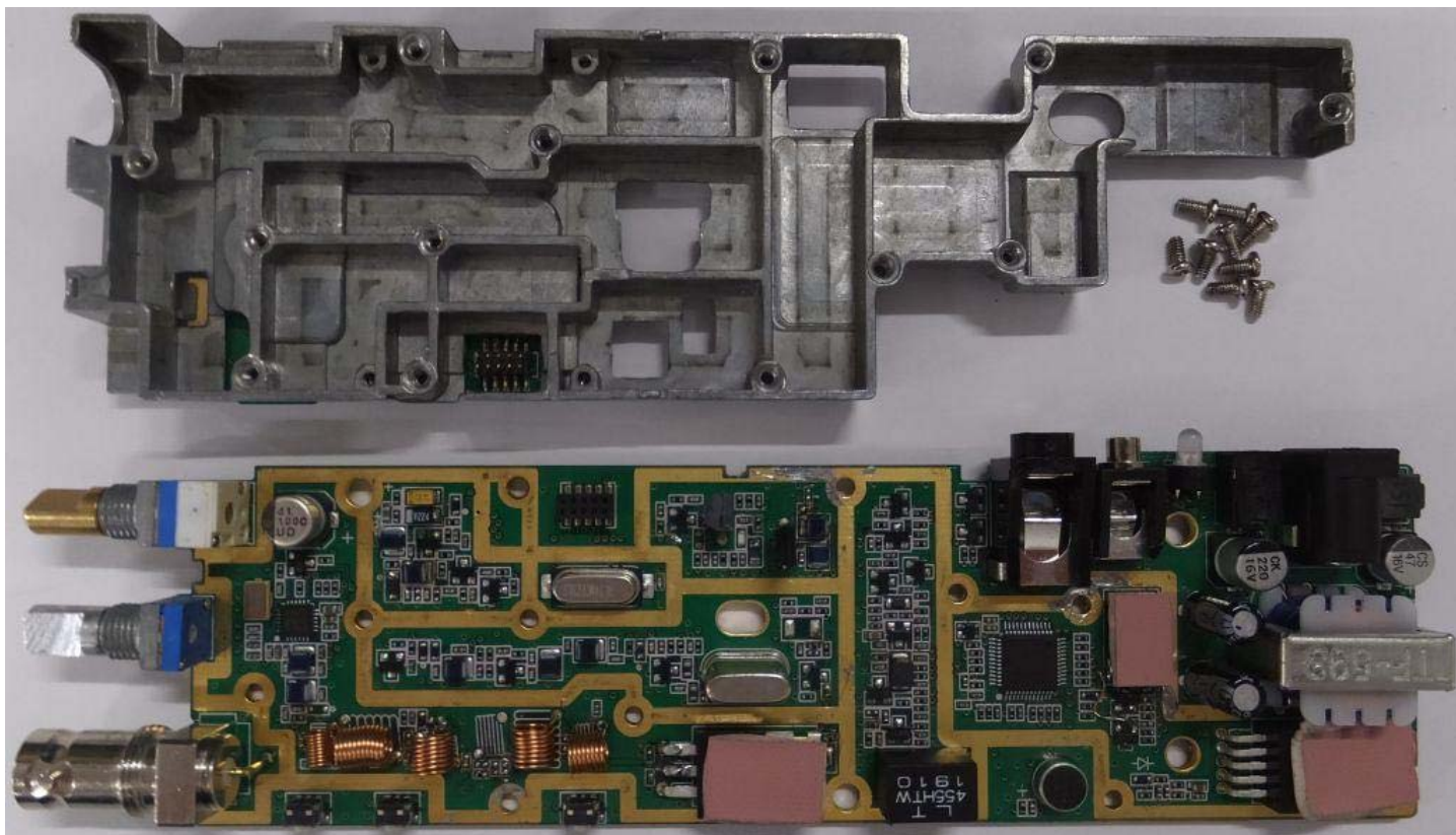
Figure E20.6 – Internal Photo – Main PCB Component Side – Heat Sink Removed-Shield Removed
