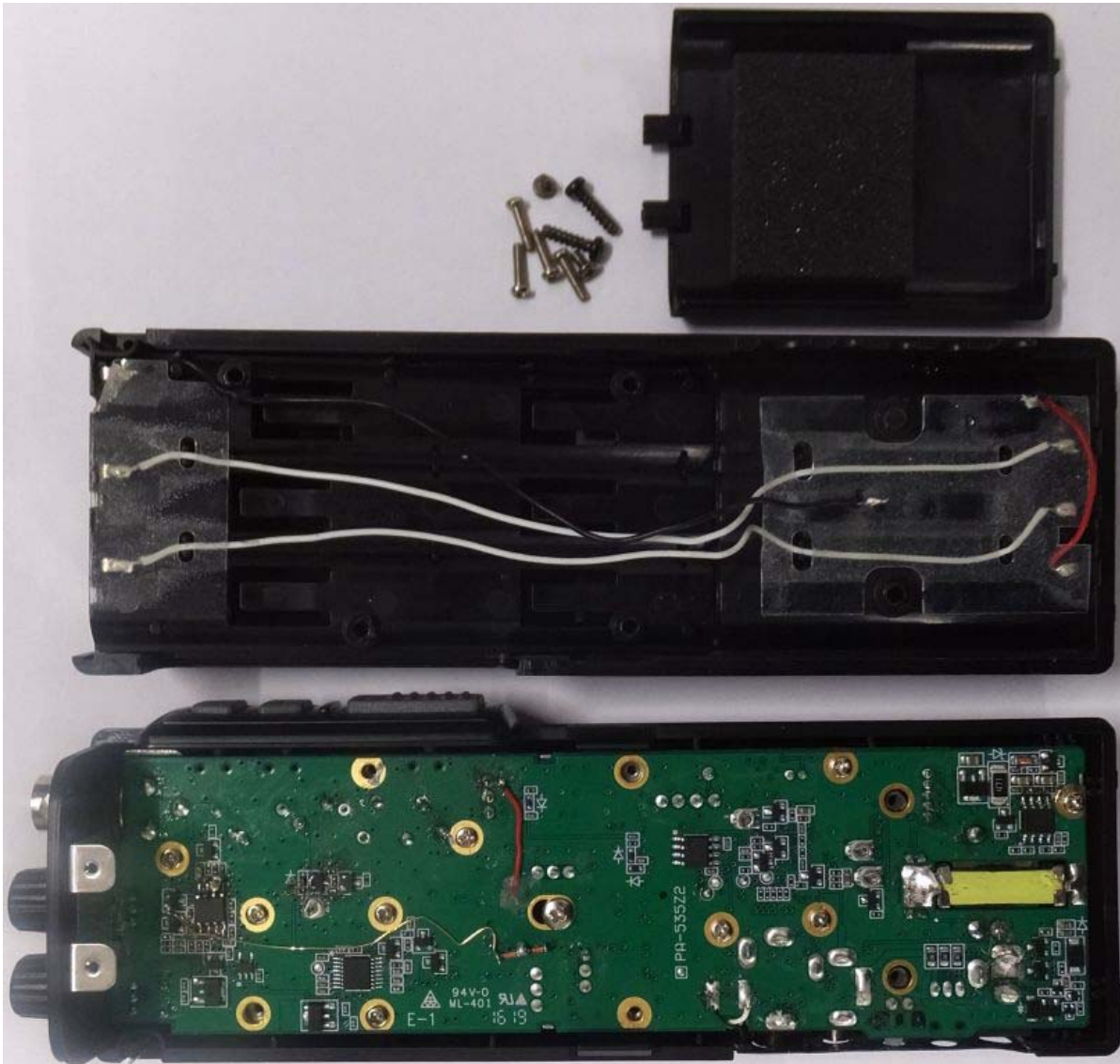
Figure E20.1 – Internal Photo – Back Cover / PCB Removed
