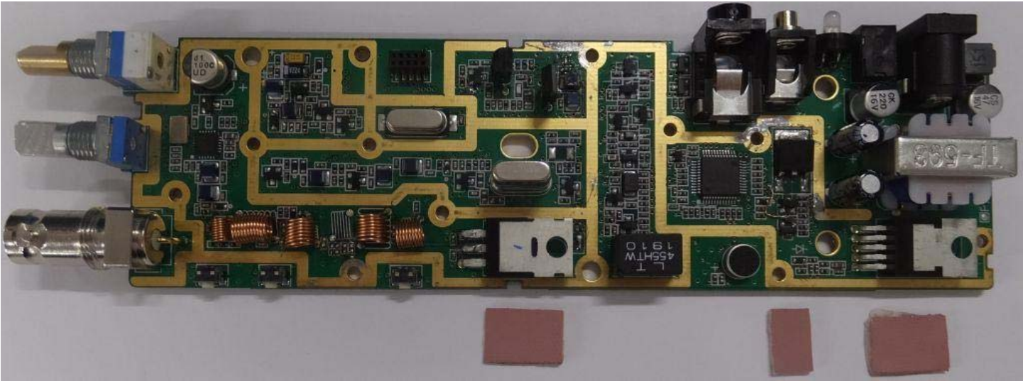
Figure E20.7 – Internal Photo – Main PCB Component Side – Heat Sink Removed-Shield Removed
