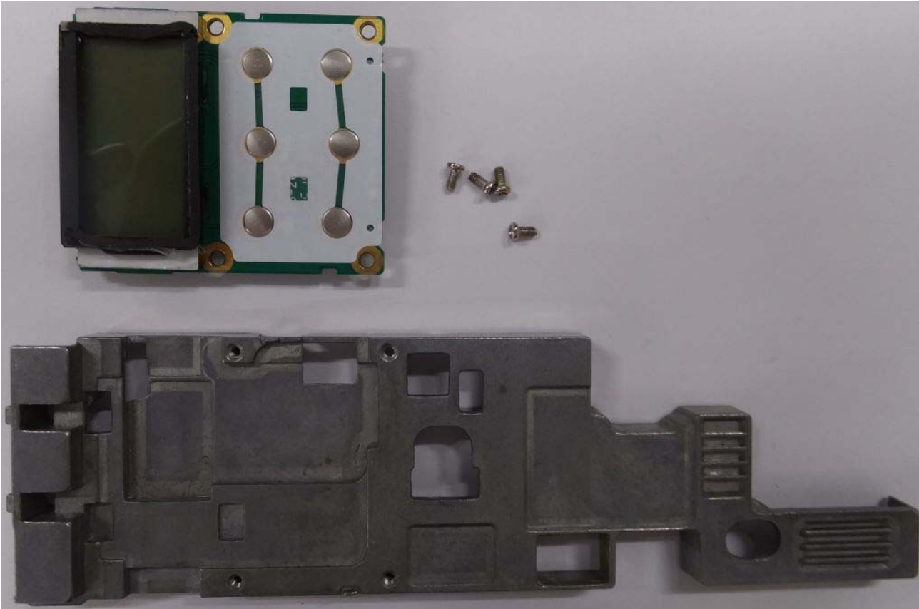
Figure E20.4 – Internal Photo – Front Cover Removed – Main PCB Display Side-Heat Sink Removed
