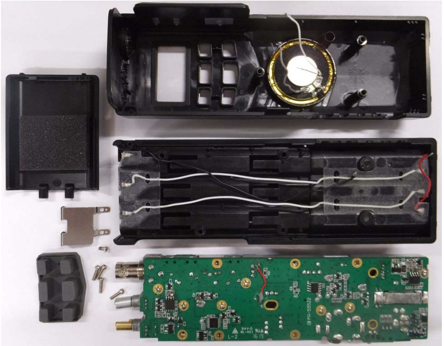
Figure E20.9 – Internal Photo – Assembly Drawing
