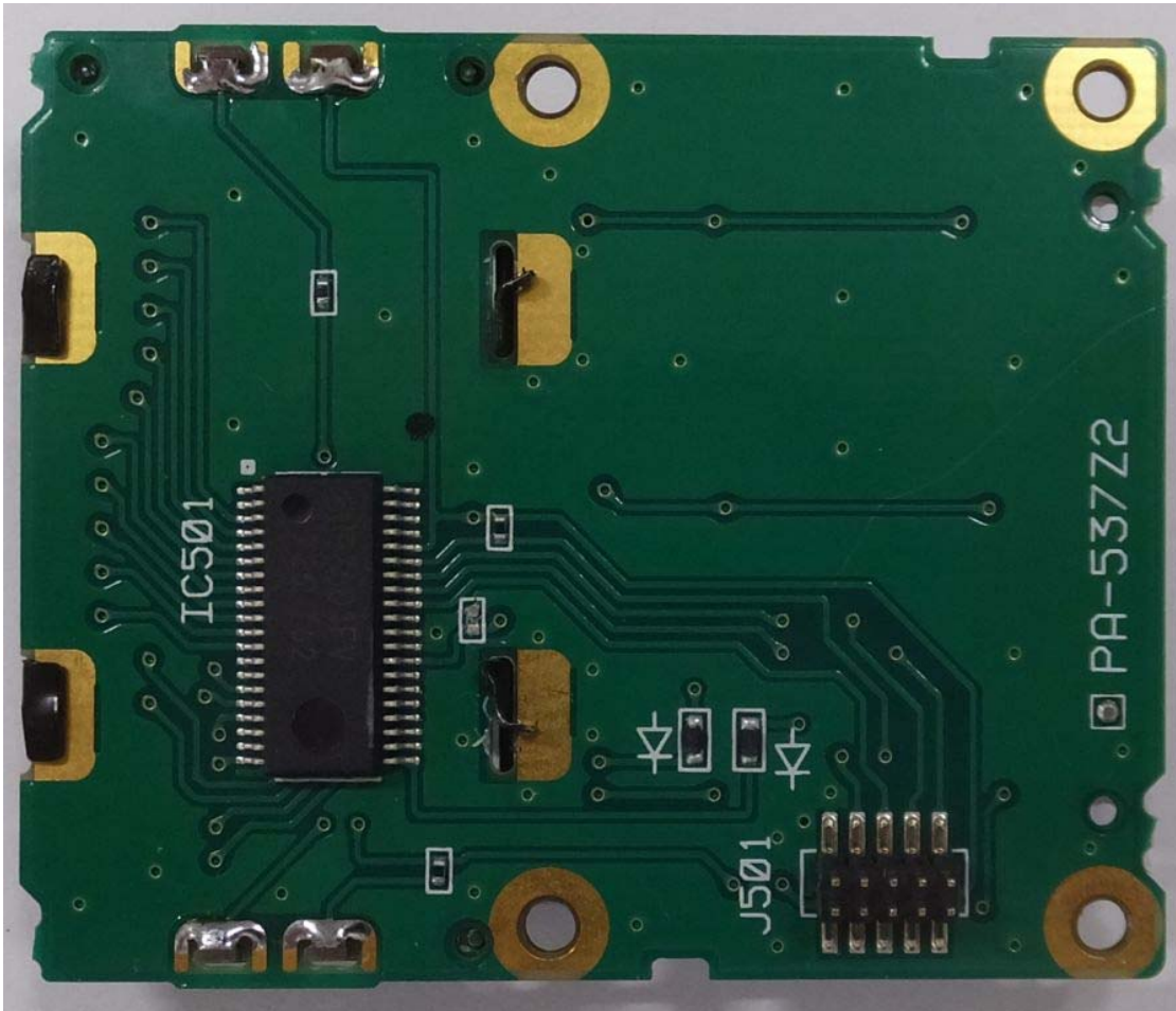
Figure E20.10 – Internal Photo – Display PCB Display Side – Display Removed
