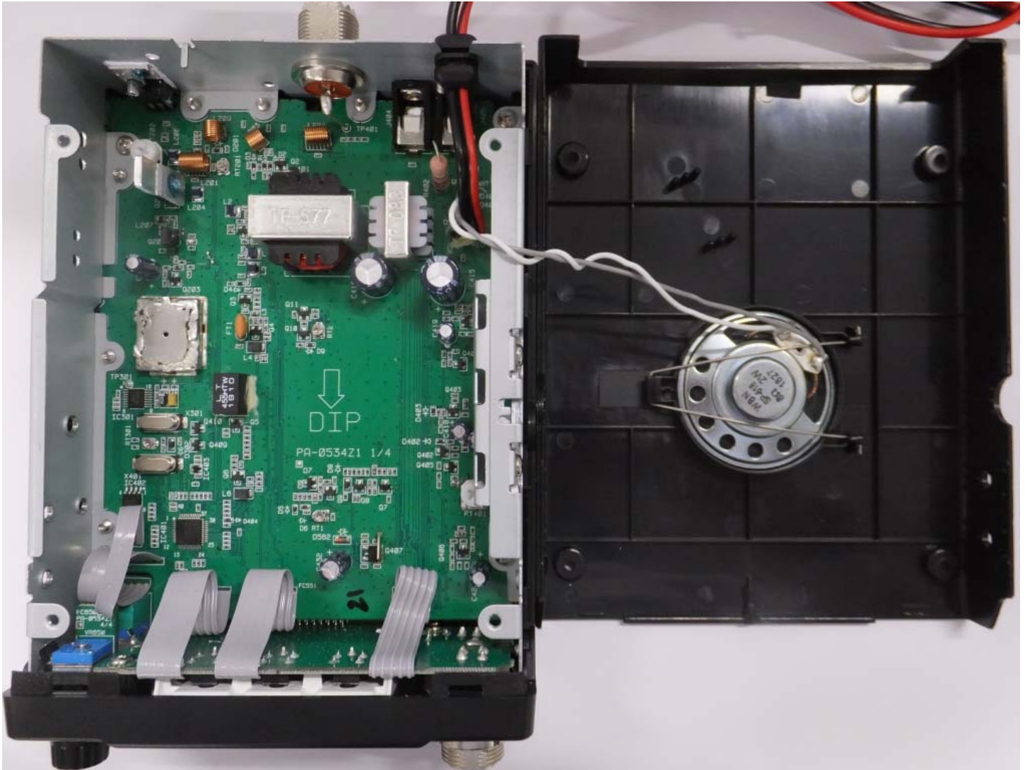
Figure E20.2 – Internal Photo – Bottom Cover Removed - PCB Component Side
