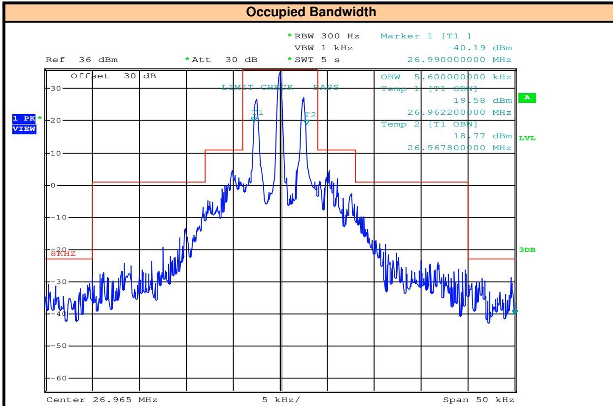
Plot 9.1 – Occupied Bandwidth Channel 1
