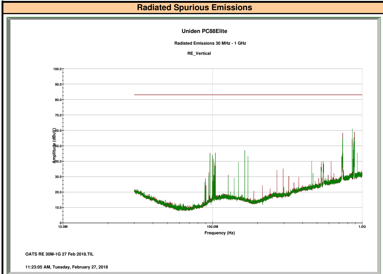
Plot 11.1 – Radiated Spurious Emissions, 30MHz – 1000MHz, Vertical
