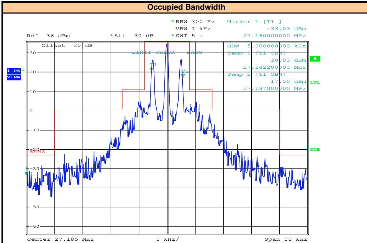
Plot 9.2 – Occupied Bandwidth Channel 19
