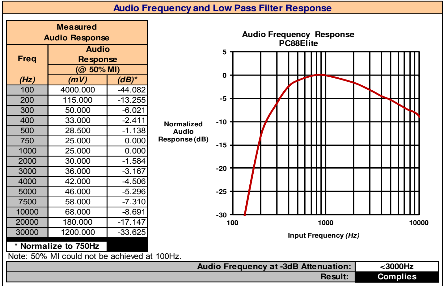
Plot 8.1 – Audio Frequency and Low Pass Filter Response
