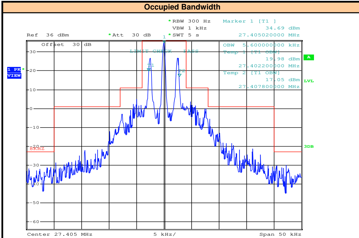
Plot 9.3 – Occupied Bandwidth Channel 40
